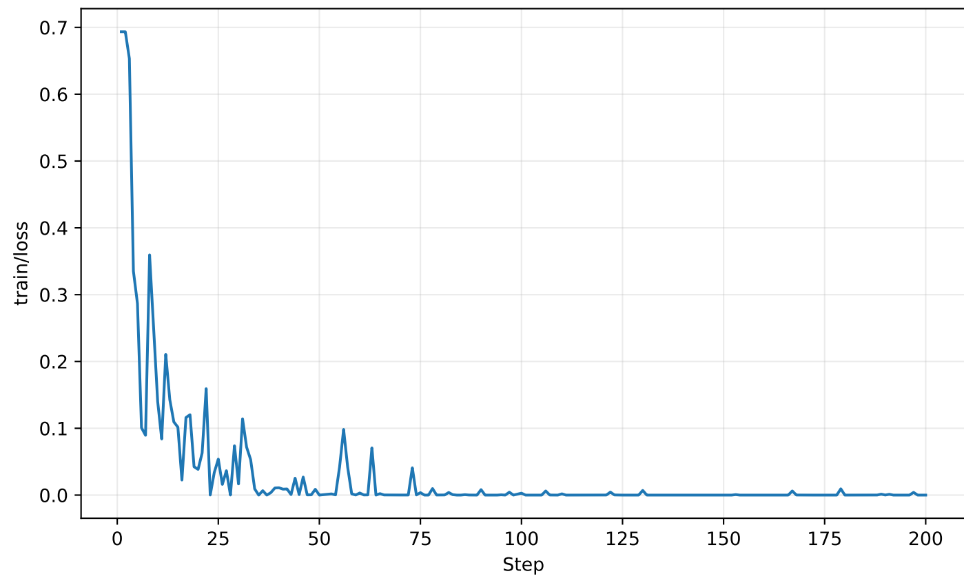
all — train/loss
