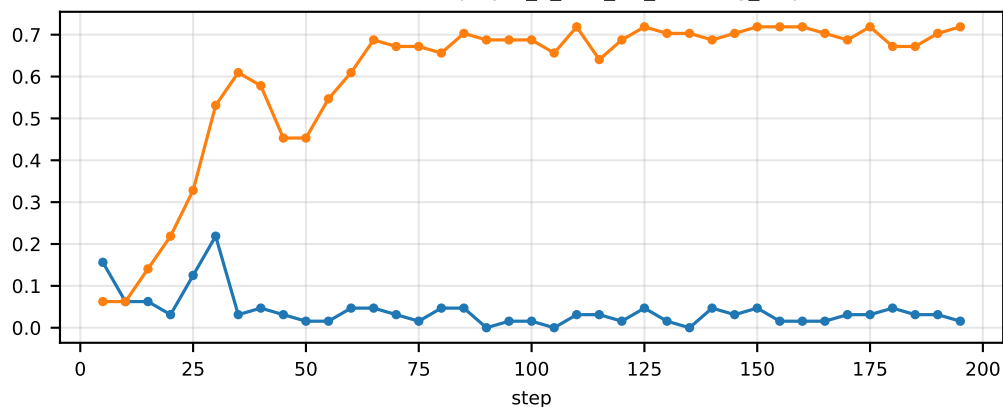
val/env/KuhnPoker-first/player_0_lose_for_wrong_format
