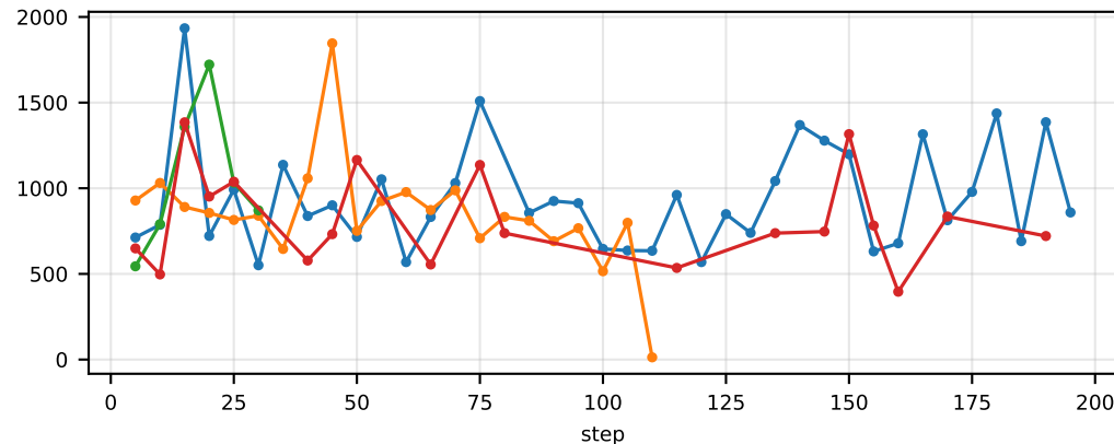
val/env/TicTacToe-second-1000/response_length_turn_3
