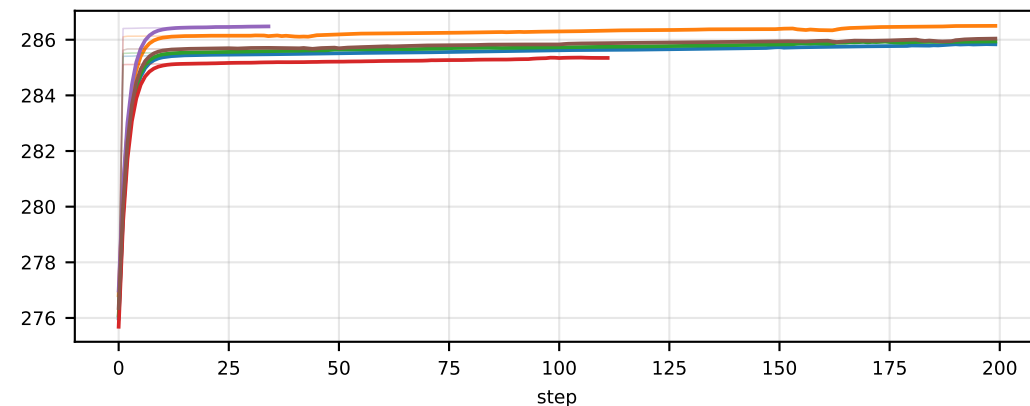
memory/cpu/actor_train/model_update/end/vms
