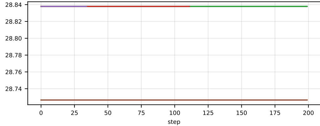
memory/reference/compute_log_probs/end/onload/reserved/0
