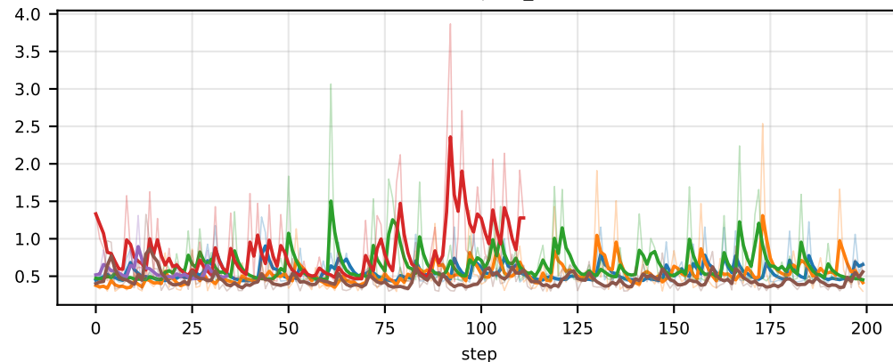
time/reference/compute_log_probs/execute
