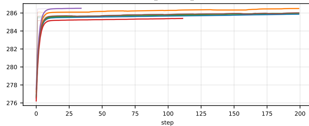
memory/cpu/reference/compute_log_probs/end/vms
