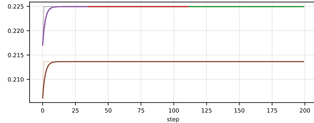
memory/actor_train/compute_log_probs/start/offload/allocated/0
