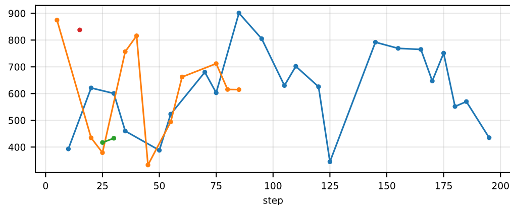
val/env/TicTacToe-second-100/winner
