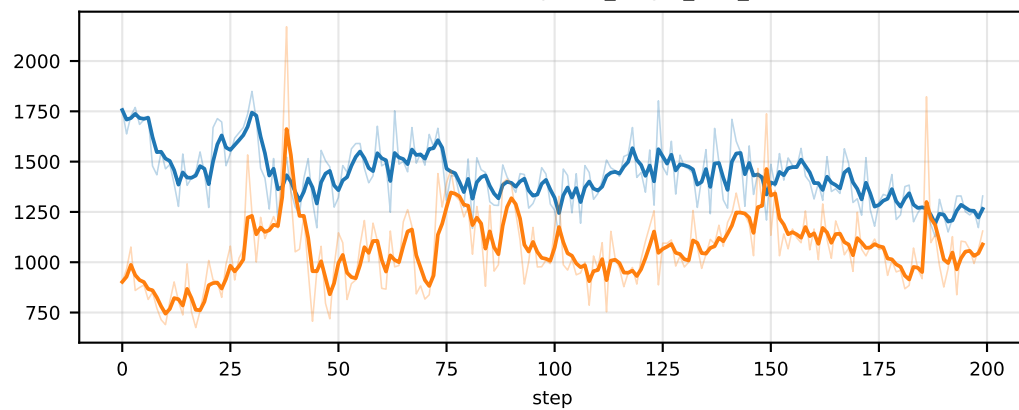
env/KuhnPoker/response_length_player_0_turn_0
