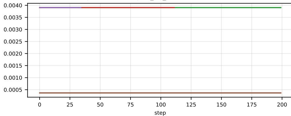
memory/reference/compute_log_probs/end/offload/max_reserved/0
