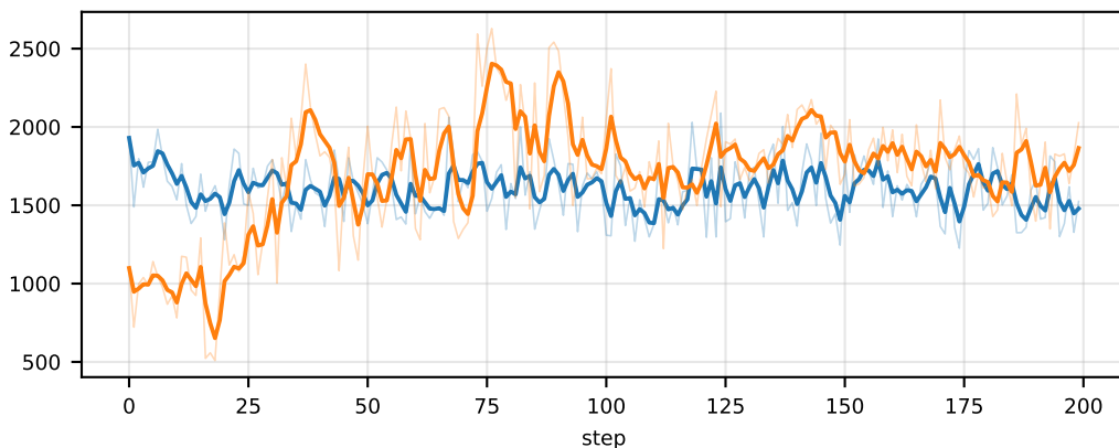
env/KuhnPoker/response_length_player_1
