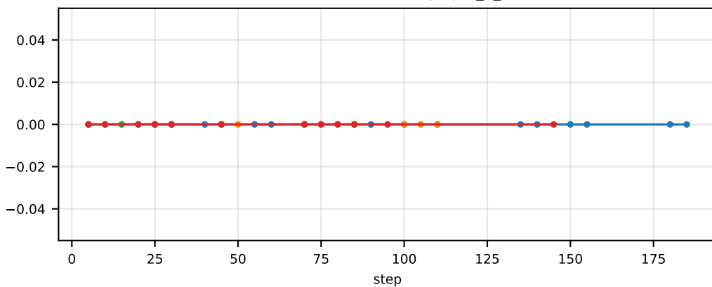
val/env/TicTacToe-first-1000/player_1_lose_for_overlong_sequence
