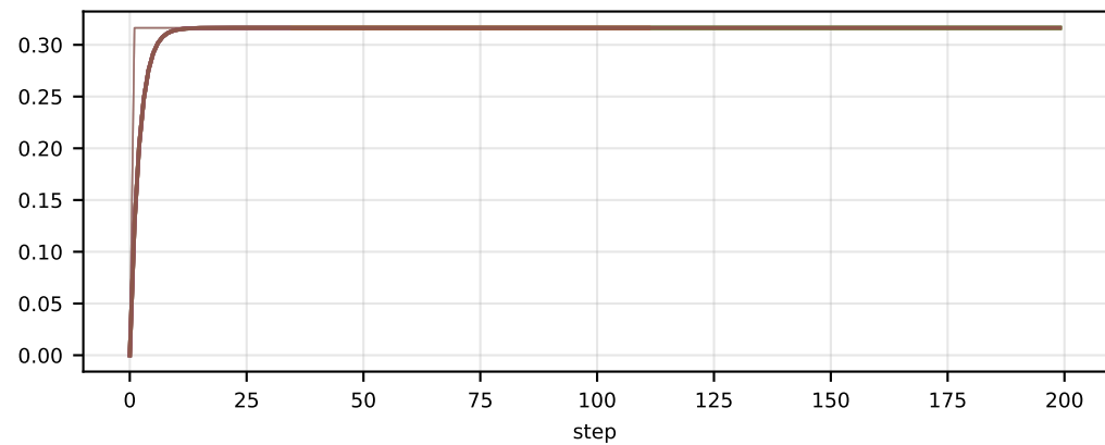
memory/actor_train/compute_log_probs/start/offload/max_allocated/0
