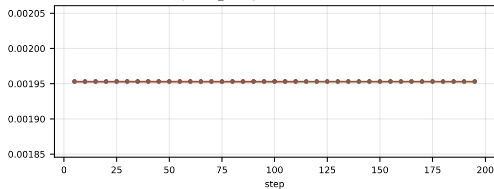
val/memory/actor_infer/generate/start/onload/reserved/0
