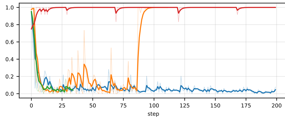
env/TicTacToe/player_1_lose_for_overlong_response
