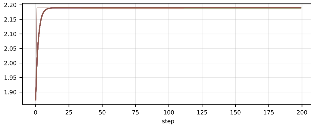
memory/actor_train/model_update/end/onload/allocated/0
