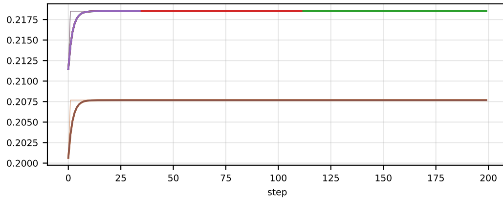
memory/actor_train/compute_log_probs/end/onload/max_reserved_frac/0
