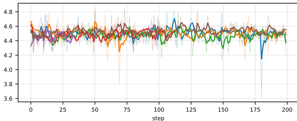
time/actor_train/model_update/onload
