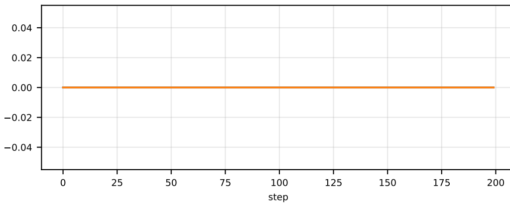
env/KuhnPoker/draw
