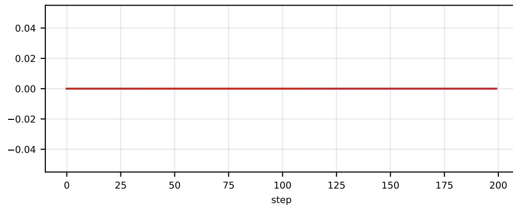
env/TicTacToe/player_1_lose_for_overlong_sequence
