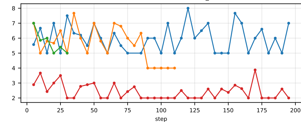
val/env/TicTacToe-second-1000/num_actions
