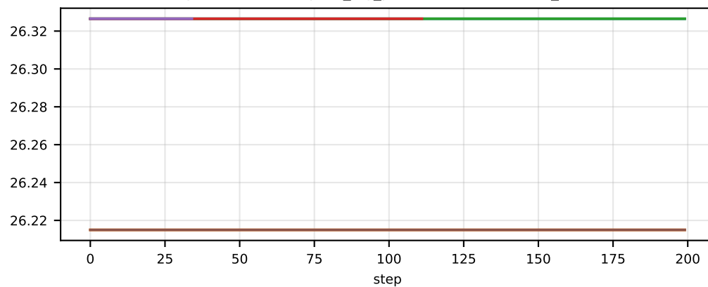
memory/reference/compute_log_probs/end/offload/reserved/0
