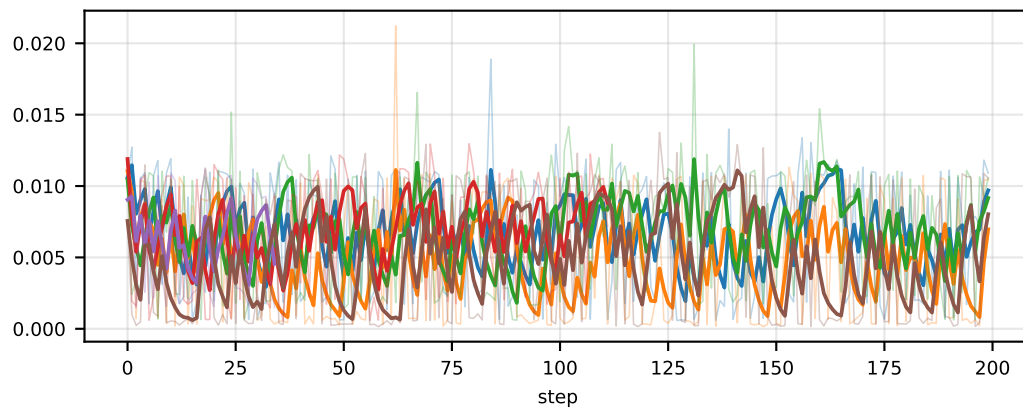
time/reference/compute_log_probs/offload
