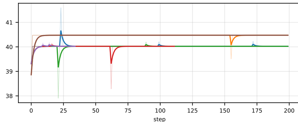
memory/actor_train/train_step/end/onload/reserved/0
