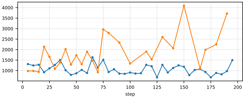
val/env/KuhnPoker-first/total_pot
