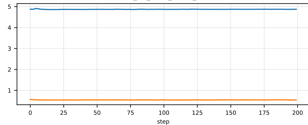
time/actor_train/train_step/total
