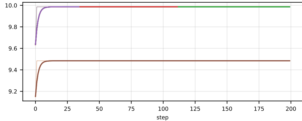
memory/actor_train/compute_log_probs/end/onload/reserved/0
