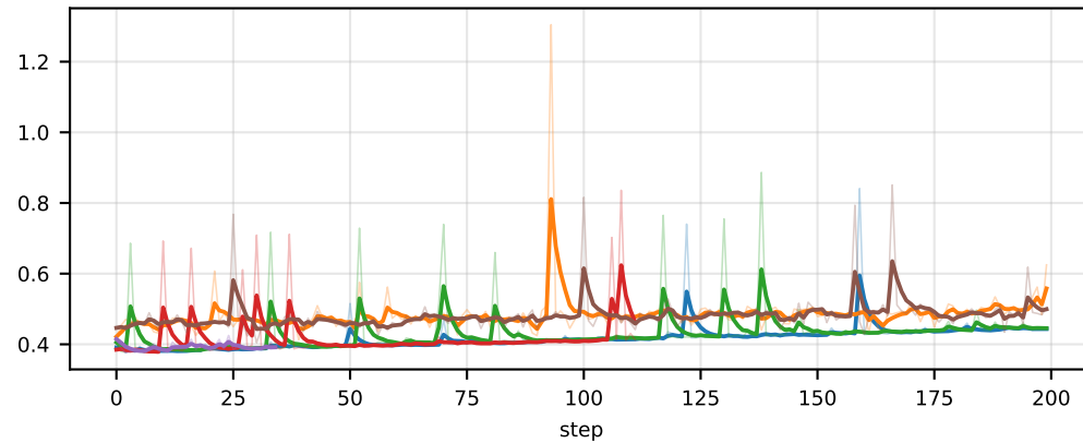
time/actor_train/train_step/onload
