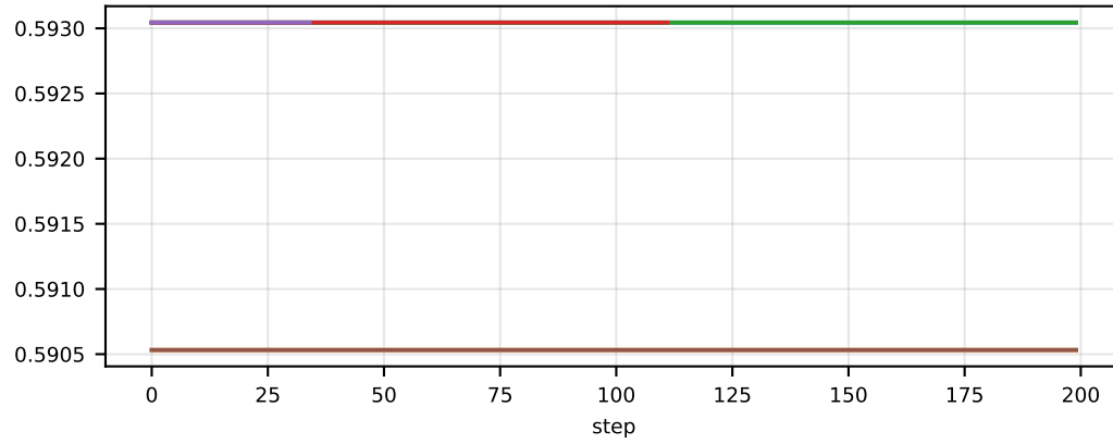
memory/reference/compute_log_probs/end/onload/max_reserved_frac/0
