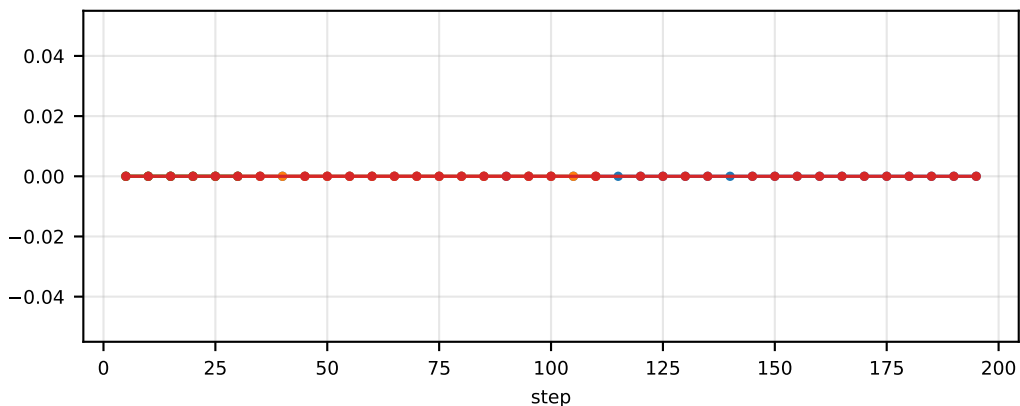
val/env/TicTacToe-first-100/player_1_success
