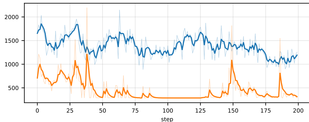
env/KuhnPoker/total_pot
