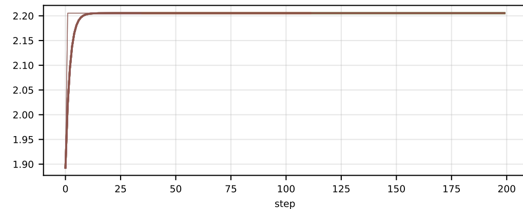
memory/actor_train/train_step/start/offload/allocated/0
