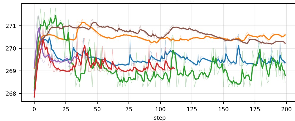
memory/reference/compute_log_probs/end/offload/max_allocated/0
