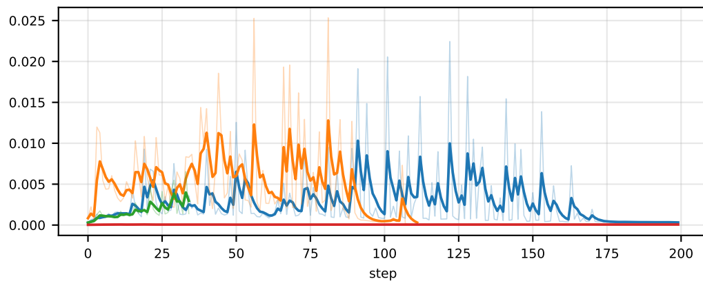
1e12 actor/ratio_max
