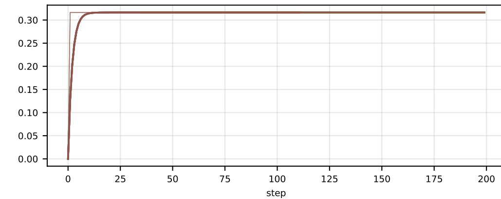
memory/actor_train/compute_log_probs/start/offload/allocated/0
