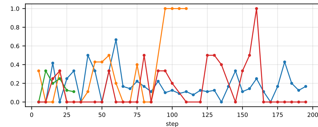
val/env/TicTacToe-first-100/winner
