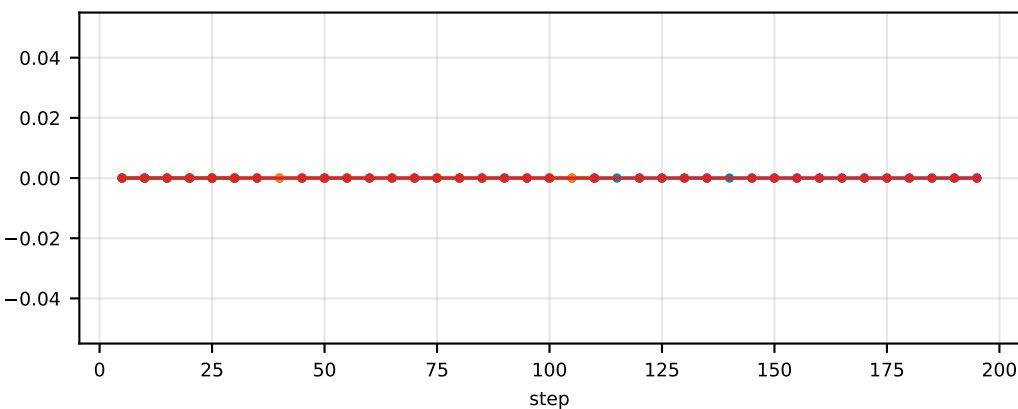
val/env/TicTacToe-first-100/success
