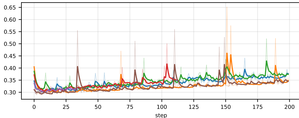
time/actor_train/do_checkpoint/load
