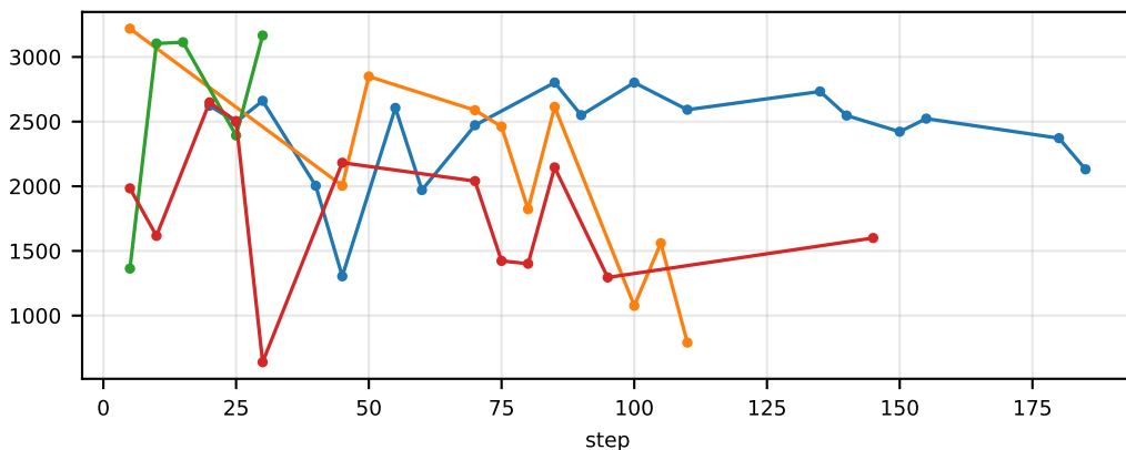
val/env/TicTacToe-first-1000/response_length_turn_0
