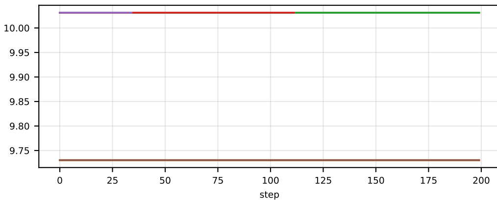
memory/actor_train/train_step/end/offload/max_reserved/0
