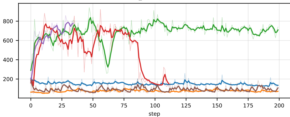
time/actor_train/compute_log_probs/offload
