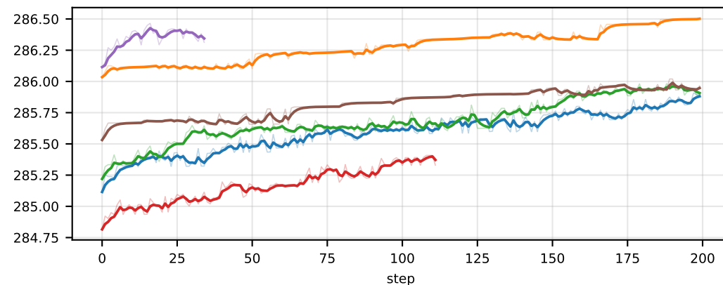
memory/cpu/actor_train/train_step/start/vms
