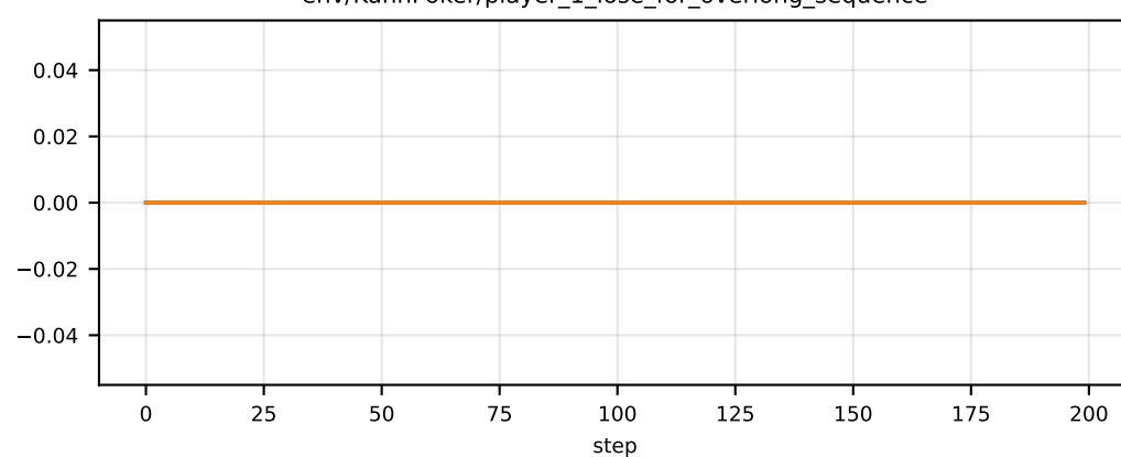
env/KuhnPoker/player_1_lose_for_overlong_sequence
