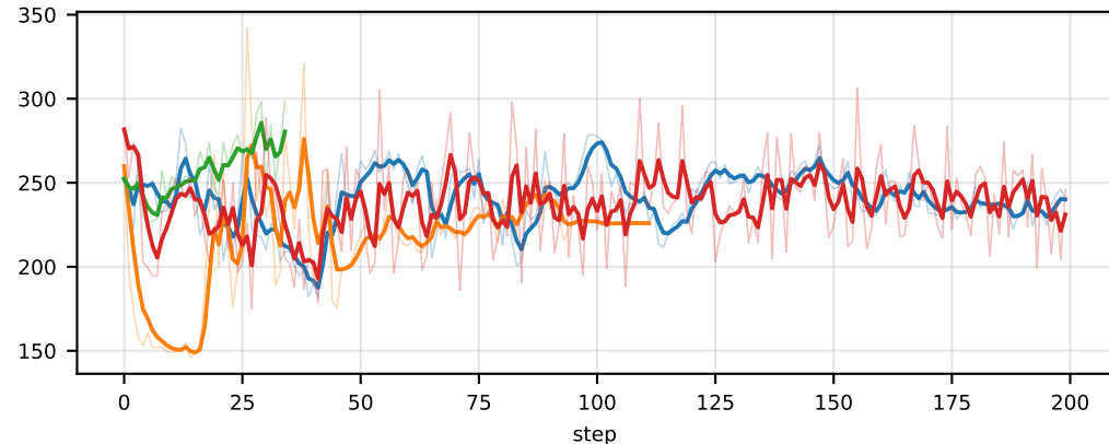
env/TicTacToe/response_length_player_0_turn_2
