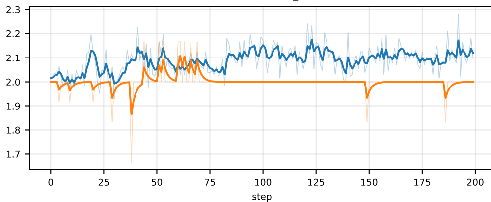
env/KuhnPoker/response_length_turn_0
