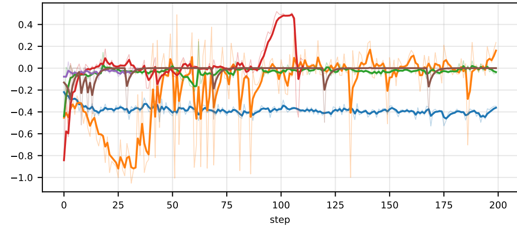
actor/total_loss
