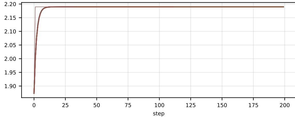
memory/actor_train/model_update/start/onload/reserved/0
