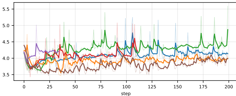
time/reference/compute_log_probs/offload
