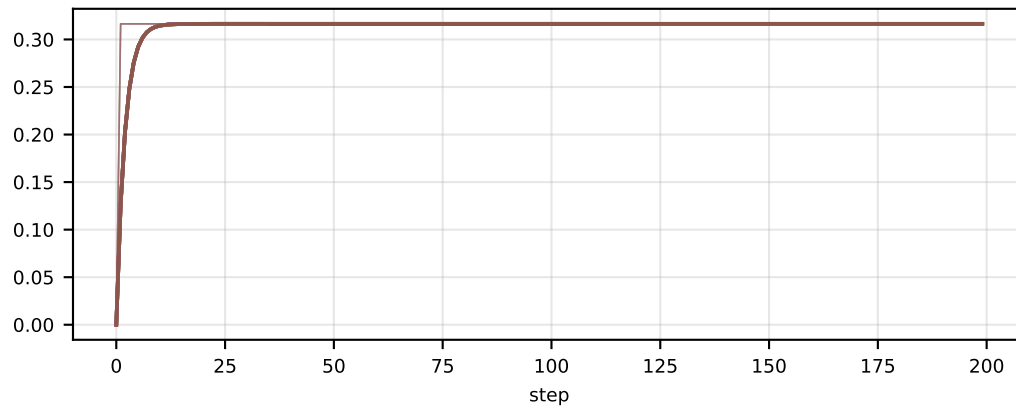
memory/actor_train/model_update/end/offload/max_reserved/0
