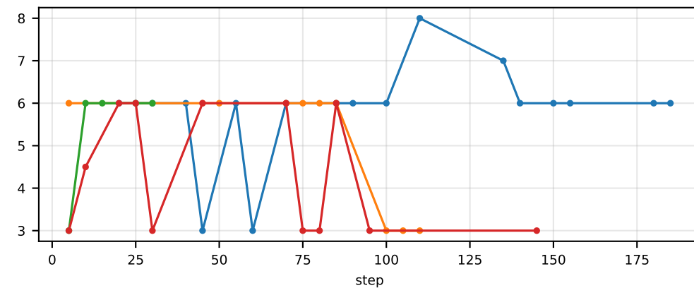
val/env/TicTacToe-first-1000/player_0_lose_for_overlong_sequence
