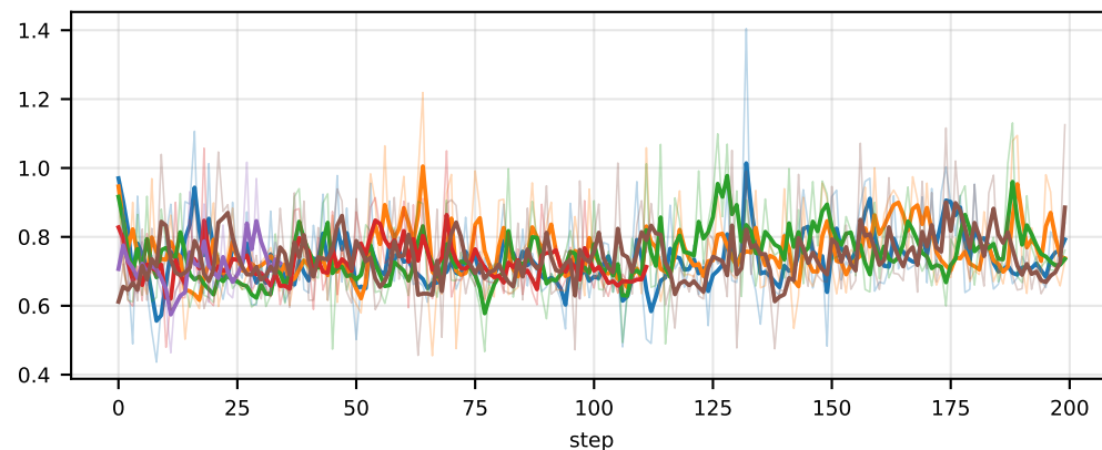
time/actor_train/train_step/execute
