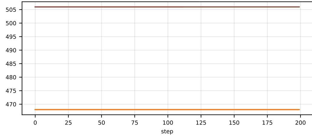
tokens/prompt_length/min
