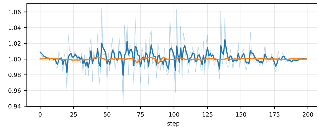
actor_train/grad_norm
