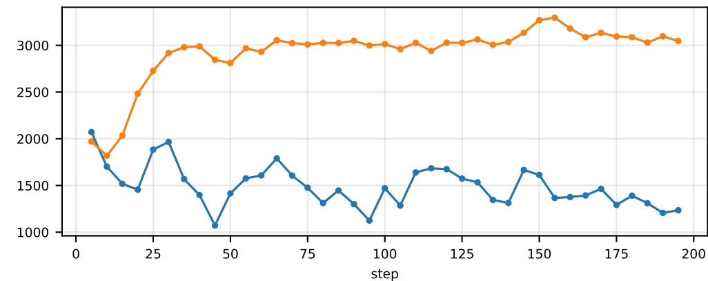
val/env/KuhnPoker-first/response_length
