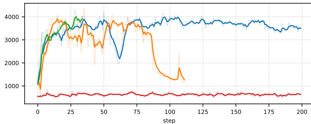
env/TicTacToe/response_length_turn_1
