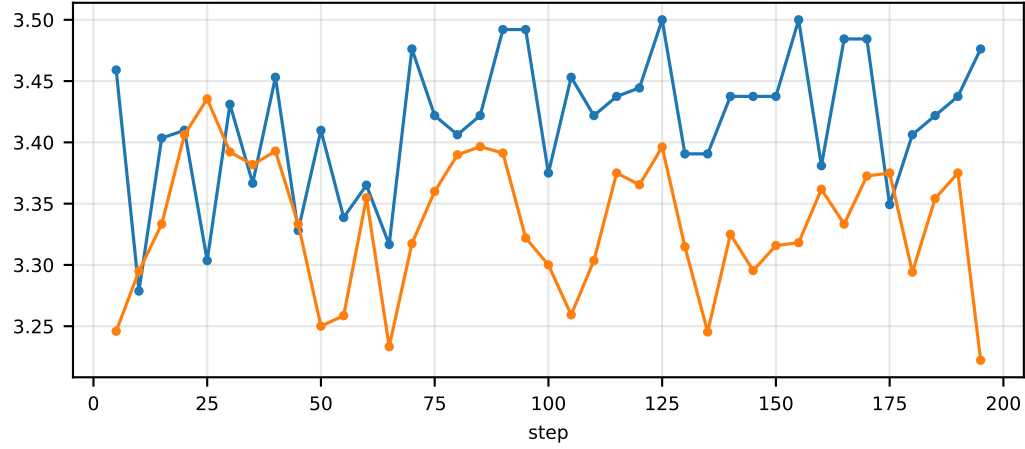
val/env/KuhnPoker-second/total_pot
