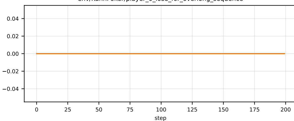
env/KuhnPoker/player_0_lose_for_overlong_sequence
