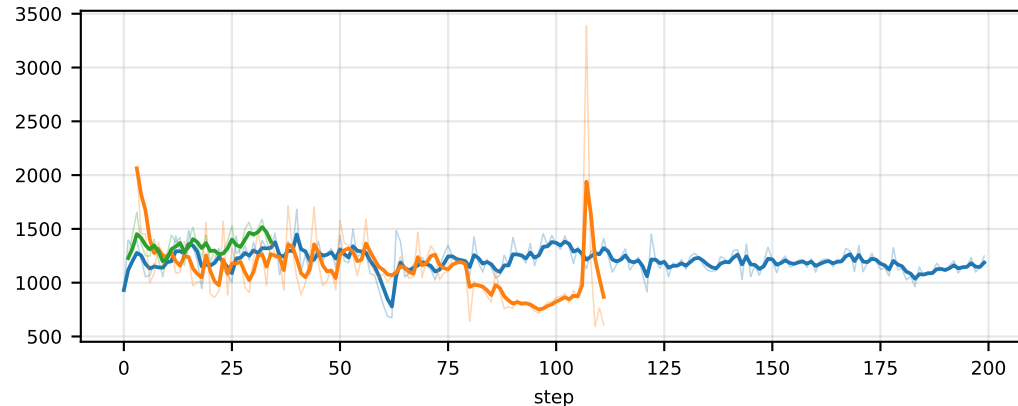
env/TicTacToe/response_length_player_1_turn_3
