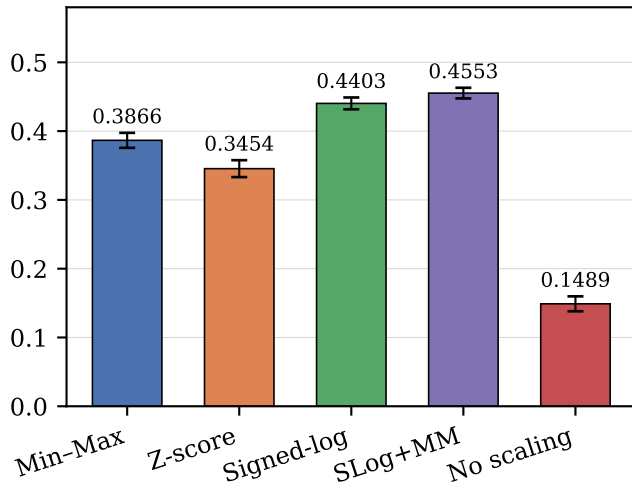
NF-UNSW-NB15-v3
