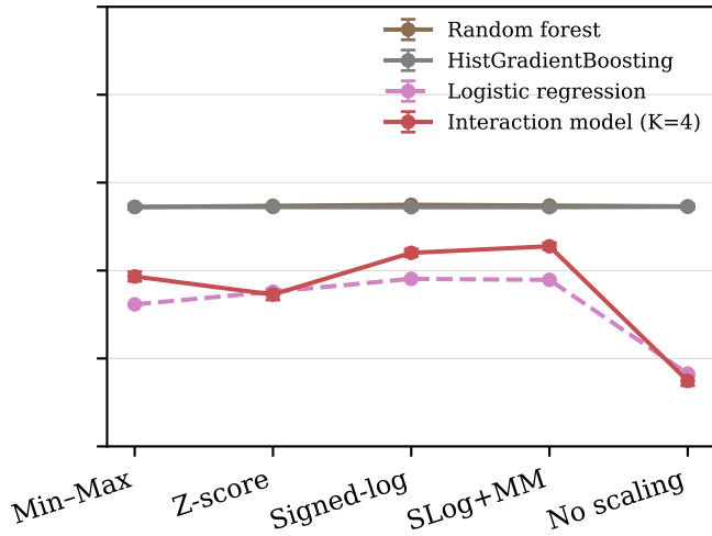
NF-UNSW-NB15-v3
