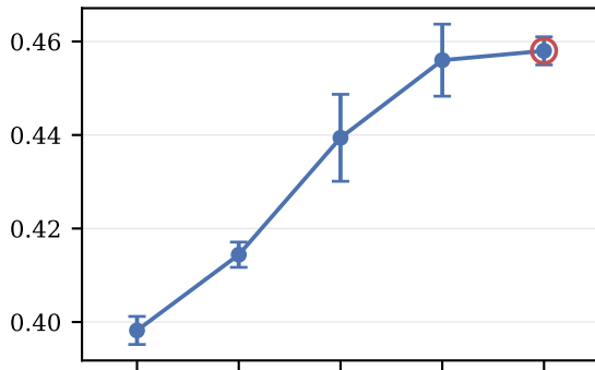
NF-UNSW-NB15-v3
