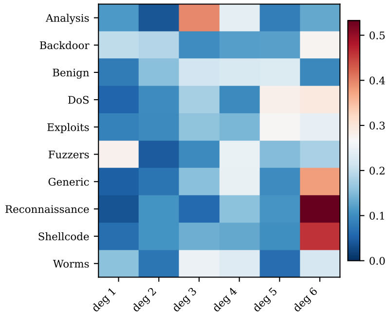
NF-UNSW-NB15-v3
