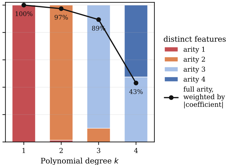
NF-UNSW-NB15-v3
