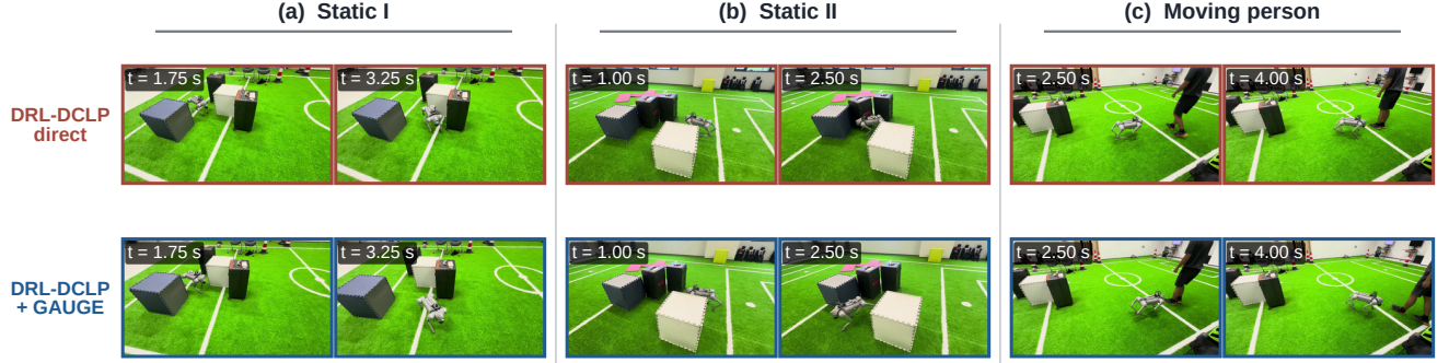
Fig. 7. Matched-time real-Go2 navigation with a fixed DRL-DCLP planner. Rows compare direct commands (red) and GAUGE-compensated commands (blue) in (a)–(b) two static-obstacle scenes and (c) a crossing-pedestrian scene. Each condition has five repetitions; the displayed sequences are representative, not independent statistical samples.
