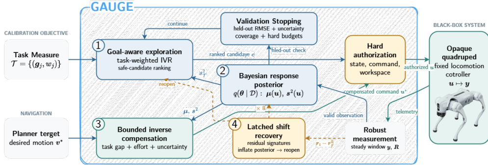
Fig. 2. GAUGE architecture. Task-weighted acquisition ranks calibration commands, but the hard filter alone authorizes execution. Valid observations update the Bayesian model; held-out validation and uncertainty control stopping. A latched residual alarm inflates posterior uncertainty and opens a bounded active-recovery phase. The inverse compensator uses the same bounded command set during navigation.
