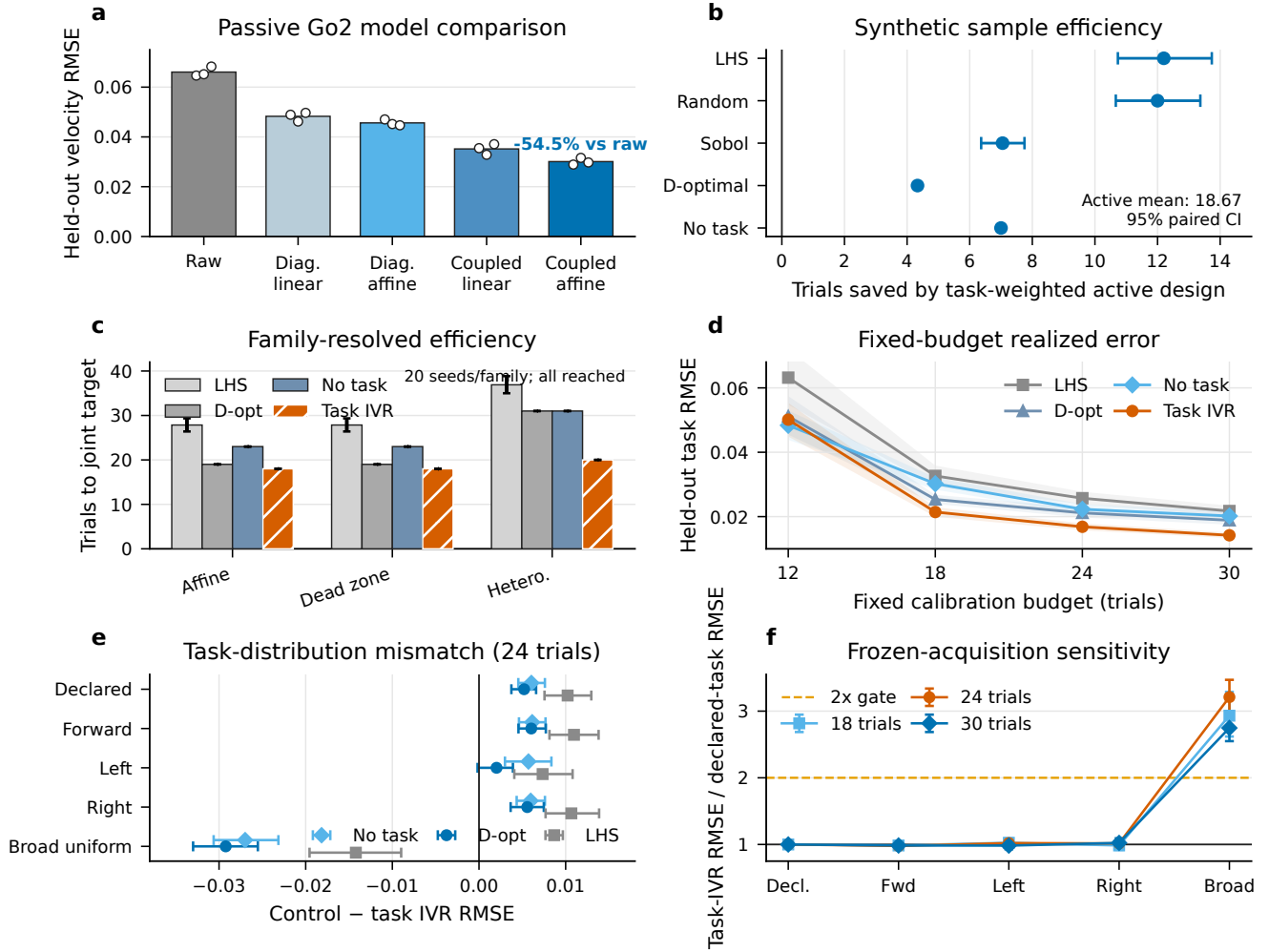
Fig. 5. Calibration evidence. (a) Passive real-Go2 held-out RMSE for raw, diagonal-affine, and coupled-affine commands. (b) Paired trials saved by task IVR; bars are 95% seed-bootstrap intervals. (c) Family-resolved time to the same joint target; every method reaches it in all 20 seeds per family. (d) Realized held-out task RMSE at matched trial budgets; bands are 95% paired-seed bootstrap intervals. (e) Frozen-acquisition performance under task-distribution mismatch at 24 trials; positive control-minus-task-IVR values favor task IVR. (f) Task-IVR error relative to the declared measure; the uniform safe-envelope negative control crosses the pre-specified 2\times sensitivity gate.
