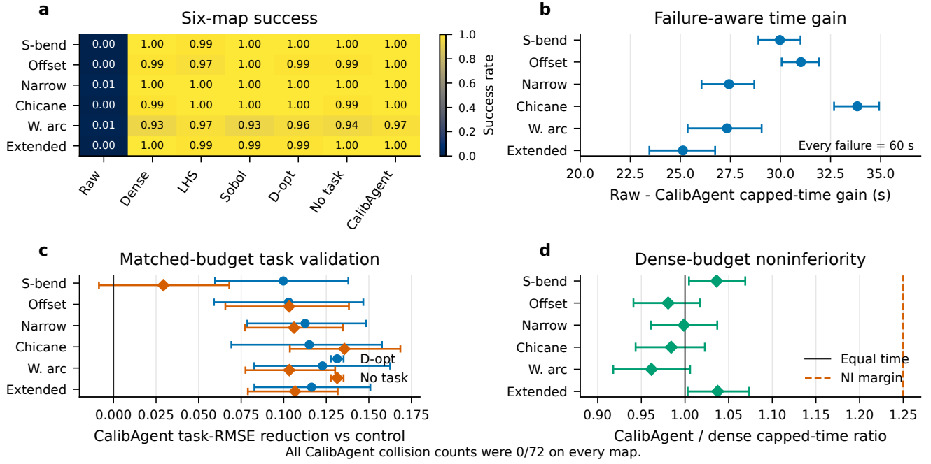
Fig. 6. Held-out simulator navigation (72 seeds/cell). (a) Success rate. (b) Paired raw-minus-CALIBAGENT gain in the 60-s capped-time estimand, which retains every failure as 60 s. (c) Matched-budget validation-RMSE reduction from task IVR relative to D-optimal and no-task IVR; bars are paired 95% intervals. (d) CALIBAGENT/dense capped-time ratios and the declared 1.25 noninferiority margin. Every CALIBAGENT collision count is 0/72.
