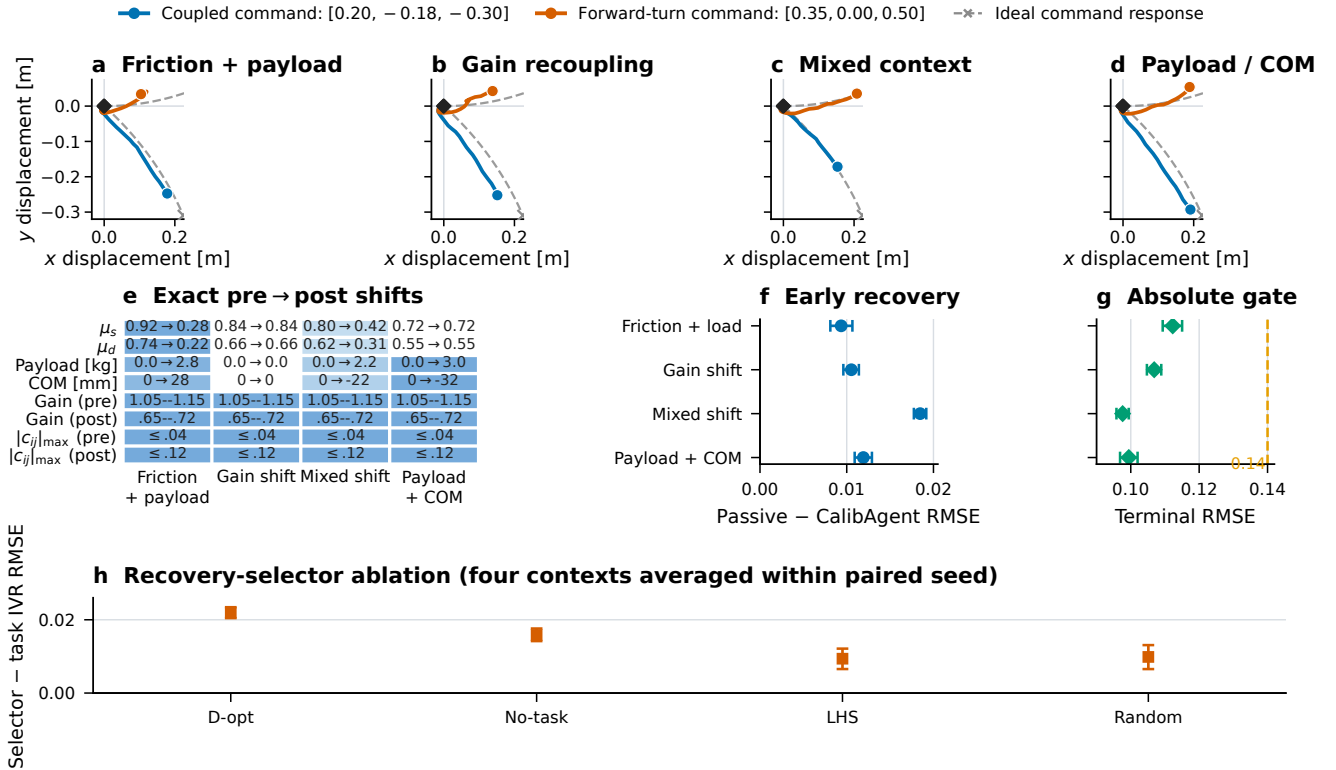
Fig. 4. Held-out simulator shifts and active recovery. (a)–(d) Measured body-displacement trajectories and dashed ideal command responses for the same validation commands in a representative paired run. (e) Exact pre→post static and dynamic friction, payload, fore-aft COM, per-axis gain range, and maximum off-axis coupling. Blue cells identify altered quantities, and every cell gives the exact pre- or post-shift value. The mixed condition additionally introduces dead zones, saturation, lag, and observation noise. (f) CALIBAGENT improvement over passive updating in the pre-specified early window. (g) CALIBAGENT terminal RMSE and the declared 0.14 gate. (h) Recovery-selector ablation (four contexts averaged within paired seed); positive values favor task IVR. Error bars are paired 95% 4,000-sample bootstrap intervals. Recovery inference pools two disjoint 72-seed blocks per shift; stationary false alarms are evaluated separately over 120 sequences and 12,000 trials.
