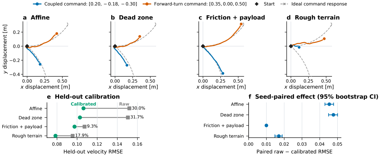
Fig. 3. Closed-loop simulation responses and calibration. (a)–(d) Body-displacement trajectories for coupled and forward-turn validation commands in a representative paired run; colored curves are measured, dashed gray curves and crosses are the ideal response to the declared command/timing, and diamonds mark the common start. (e) Raw and calibrated held-out velocity RMSE across 20 paired seeds; labels give relative reduction. (f) Seed-paired absolute improvement with 95% 4,000-sample bootstrap intervals. The trajectories are qualitative examples; all inference uses paired summaries specified before evaluation.
