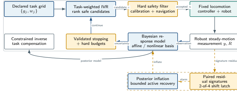
Fig. 2. GAUGE architecture. Task-weighted acquisition ranks calibration commands, but the hard filter alone authorizes execution. Valid observations update the Bayesian model; held-out validation and uncertainty control stopping. A latched residual alarm inflates posterior uncertainty and opens a bounded active-recovery phase. The inverse compensator uses the same bounded command set during navigation.
