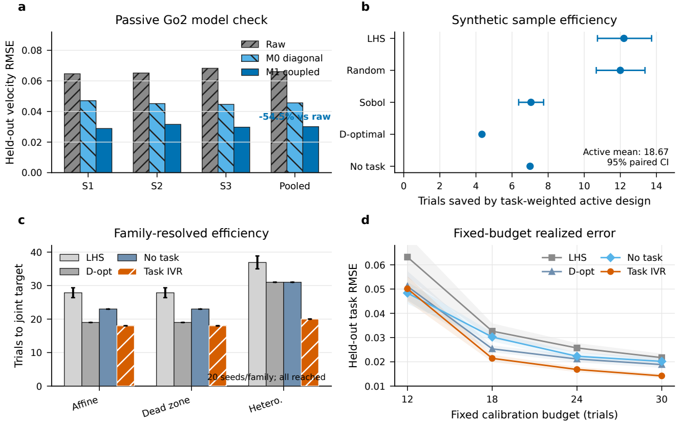
Fig. 5. Calibration evidence. (a) Passive real-Go2 held-out RMSE for raw, diagonal M0, and coupled M1 commands. (b) Paired trials saved by task IVR; bars are 95% seed-bootstrap intervals. (c) Family-resolved time to the same joint target; every method reaches it in all 20 seeds per family. (d) Realized held-out task RMSE at matched trial budgets; bands are 95% paired-seed bootstrap intervals.
