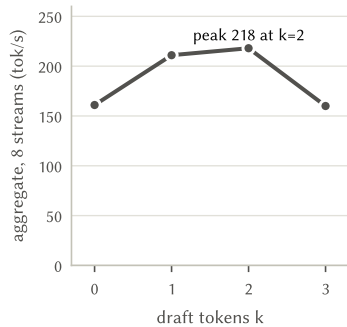
(c) Same GPU, 8 concurrent streams
