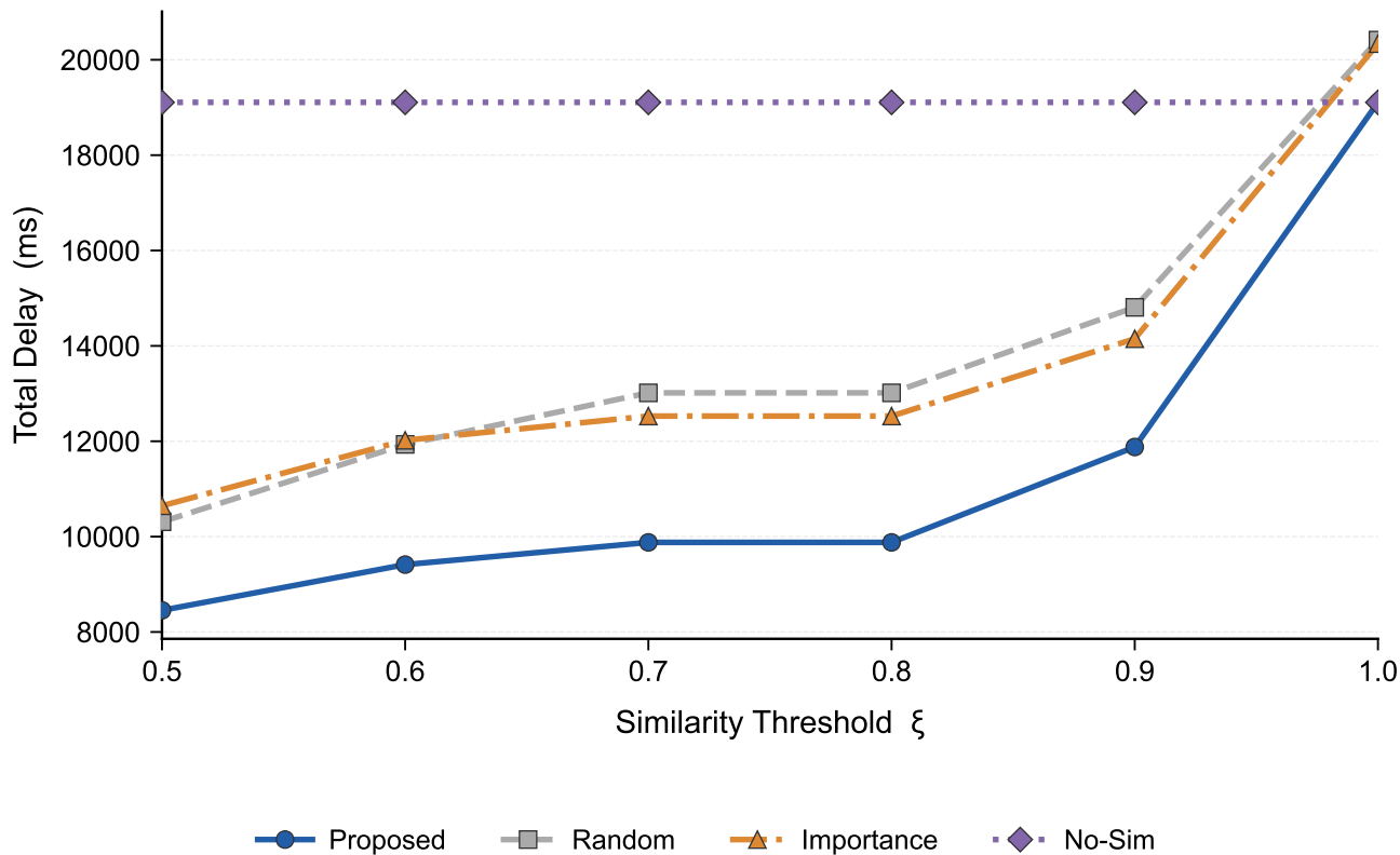
Effect of Similarity Threshold \xi
