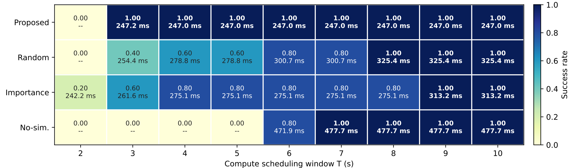
Compute Window Sensitivity: Success Rate and Per-task Delay
