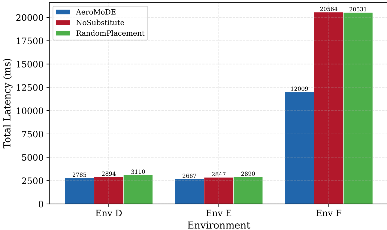
Performance on Heterogeneous UAV Environments
