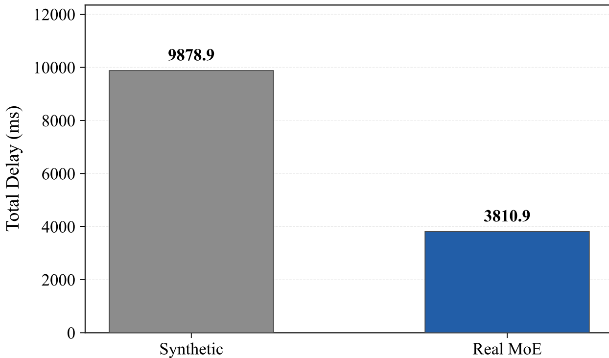
Proposed: Synthetic vs Real MoE Workload
