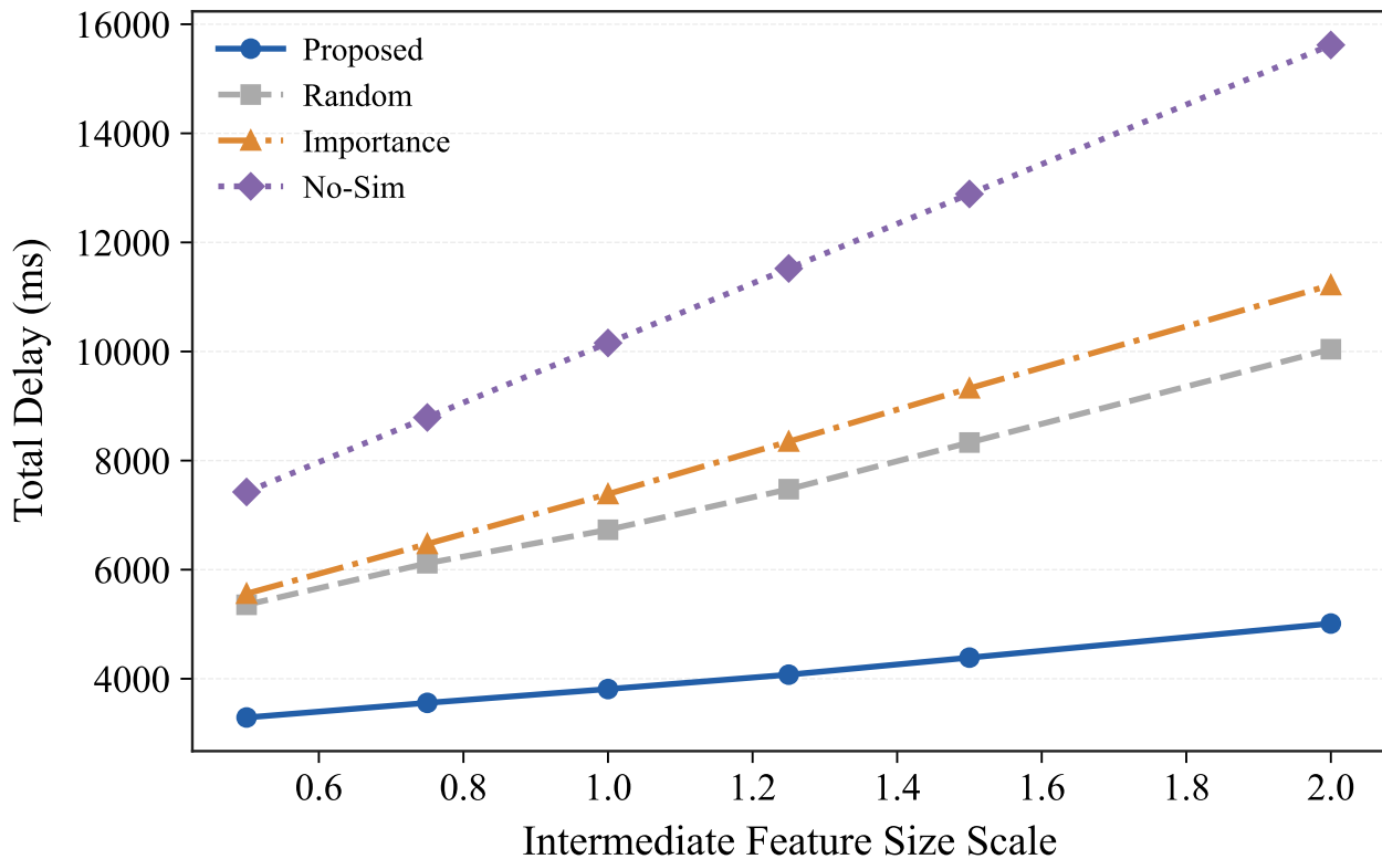
Fig. 5 Real MoE: Intermediate Feature Size
