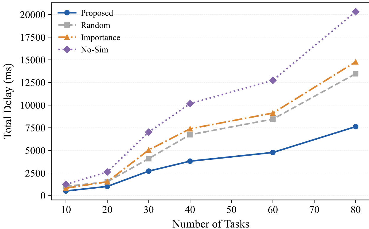
Fig. 8 Real MoE: Task Count
