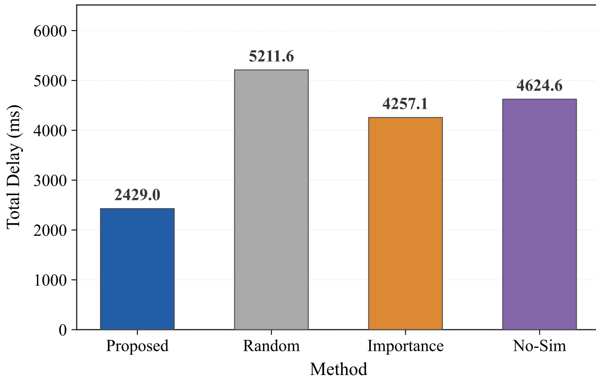
Real MoE Trace: Original Expert Size
