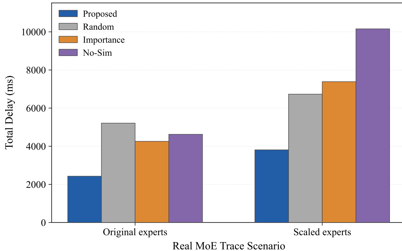
Real MoE Trace: Total Delay Under Memory Pressure
