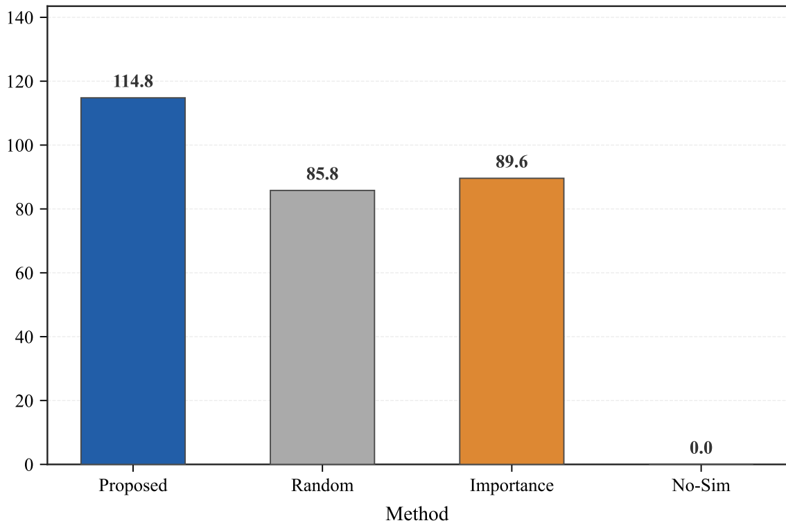
Mean Expert Substitutions
