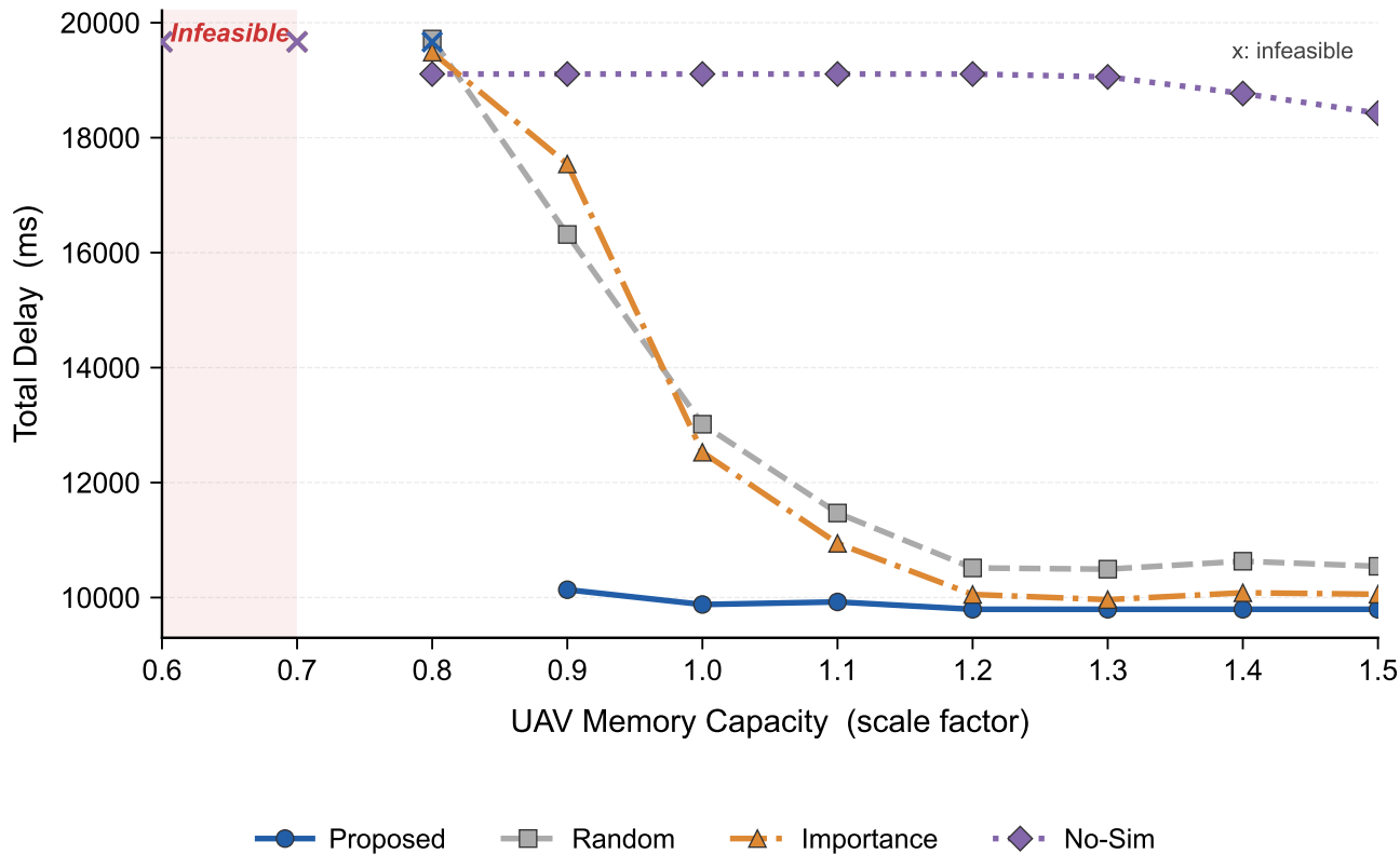
Effect of UAV Memory Capacity
