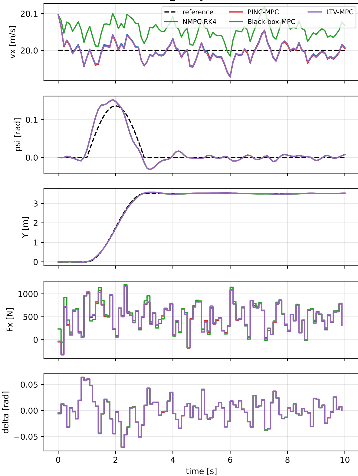
lane_change (seed 0)
