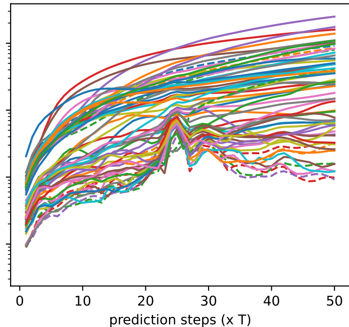
extrap
