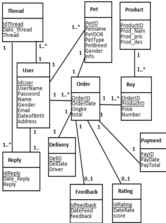
Fig. 3. Class Diagram of the proposed model
