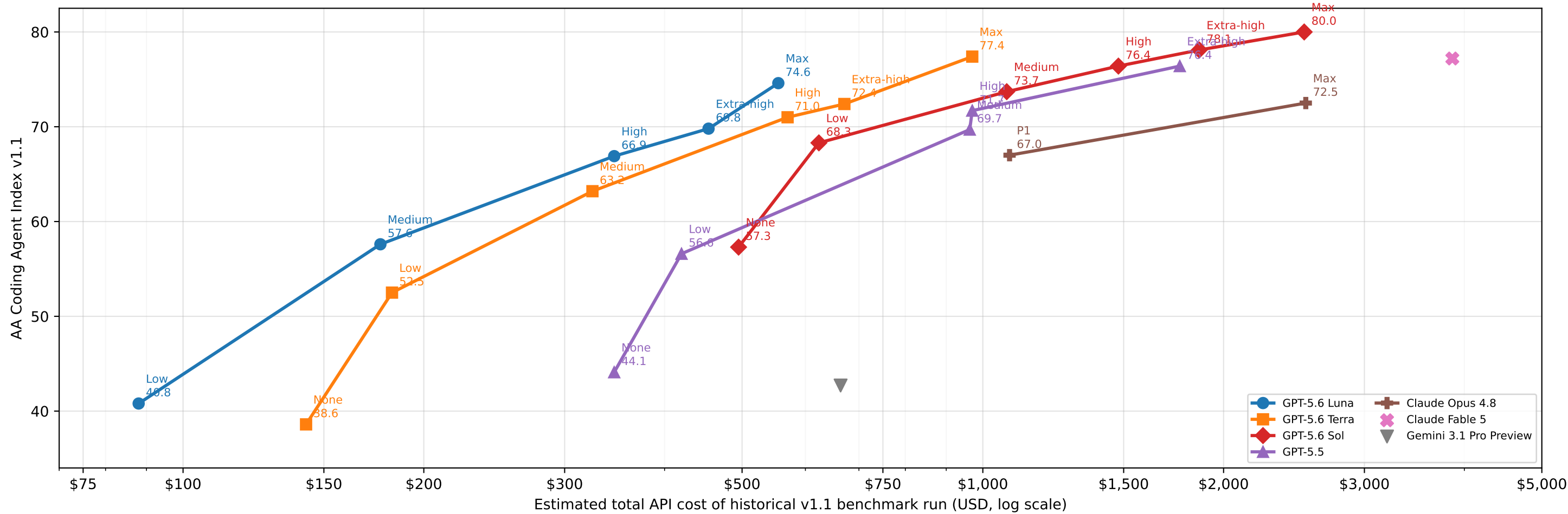
A — Historical Coding Agent Index v1.1 reconstruction
