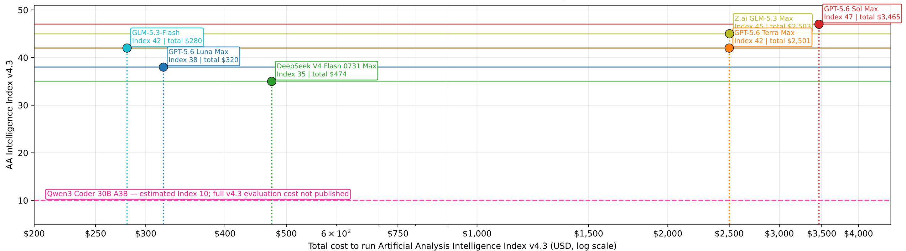
B — Current Intelligence Index vs TOTAL evaluation cost (17 Sep 2026) horizontal = index level; dotted vertical = total evaluation cost; point = measured intersection
