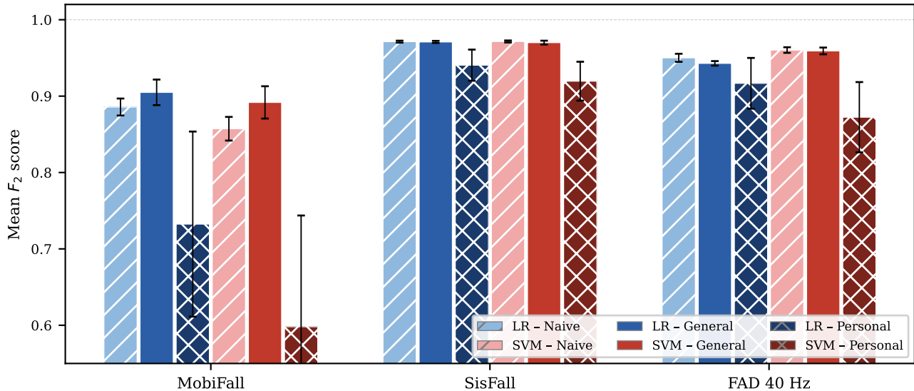
F_2 by dataset, classifier, and evaluation protocol (error bars: mean CI across subjects)
