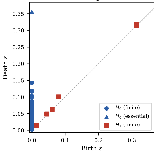
Persistence diagram — ADL
