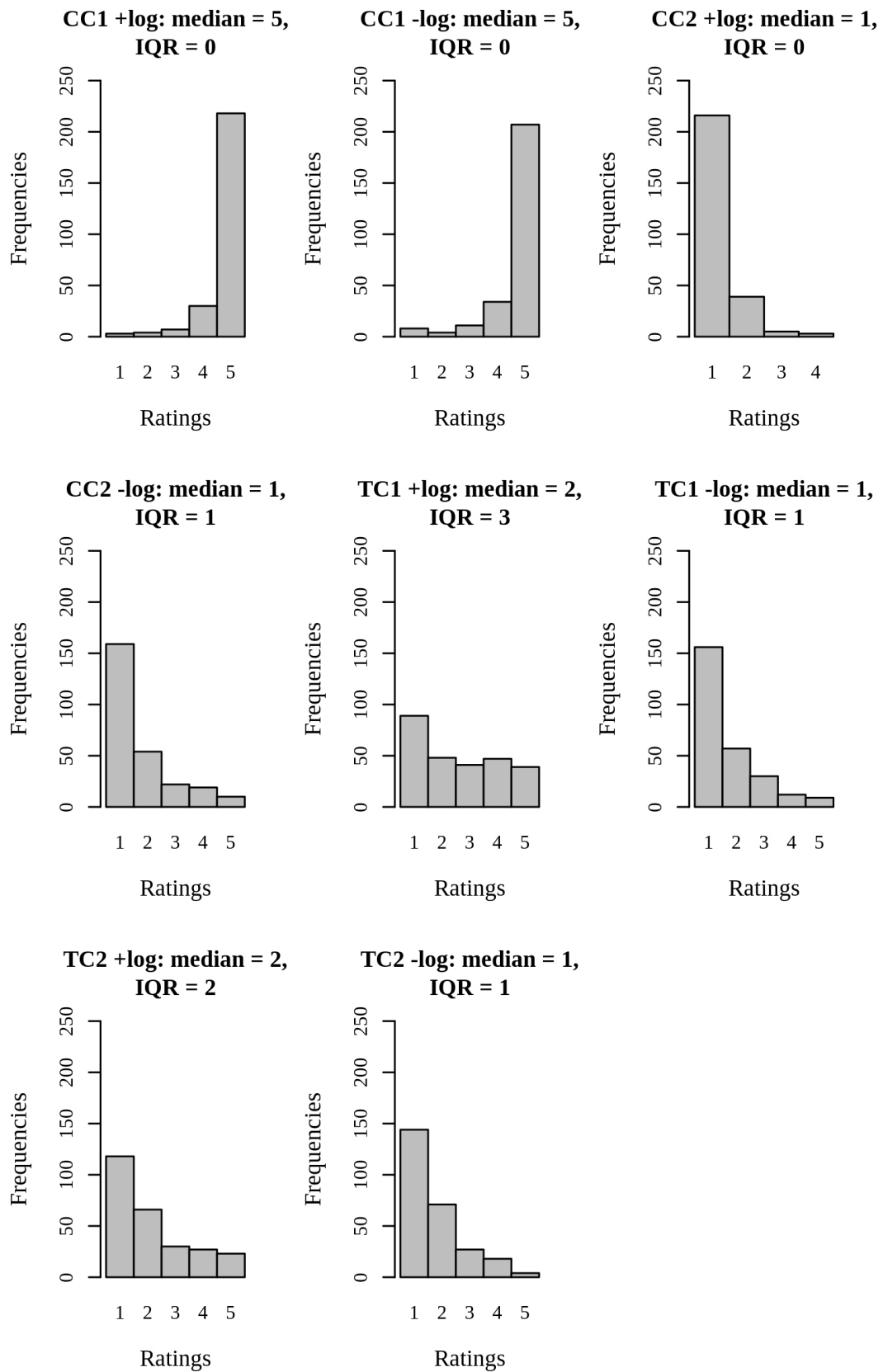
Figure 1: Descriptive statistics
