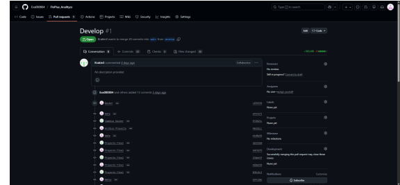
Figura 5: Pull Requests.
