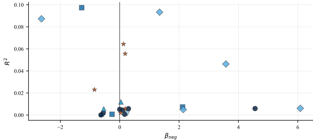
Signal Strength: \beta_{neg} vs. R^2 (ESG vs Conv.)
