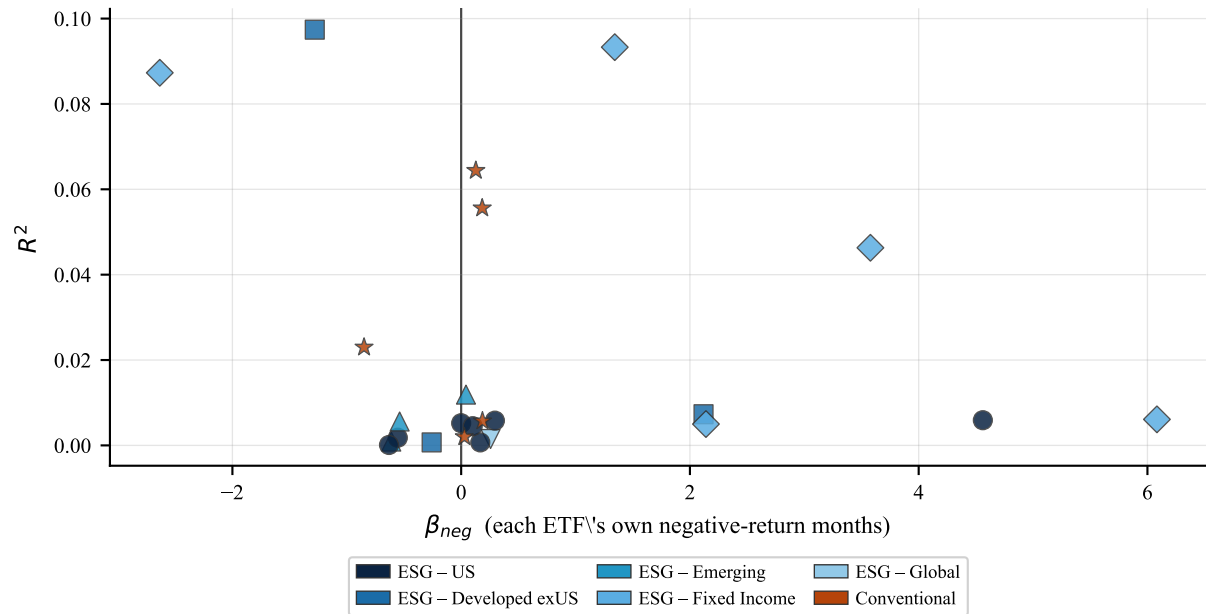
Signal Strength: \beta_{neg} vs. R^2 (ESG vs Conv.)
