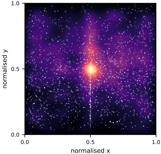
Qwen2.5-VL-7B / phantom ( n=2735 , \bar{d}=0.314 )
