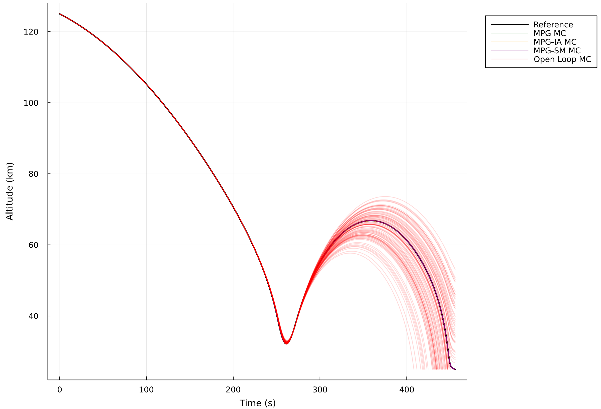
Monte Carlo Simulations: Altitude Profiles
