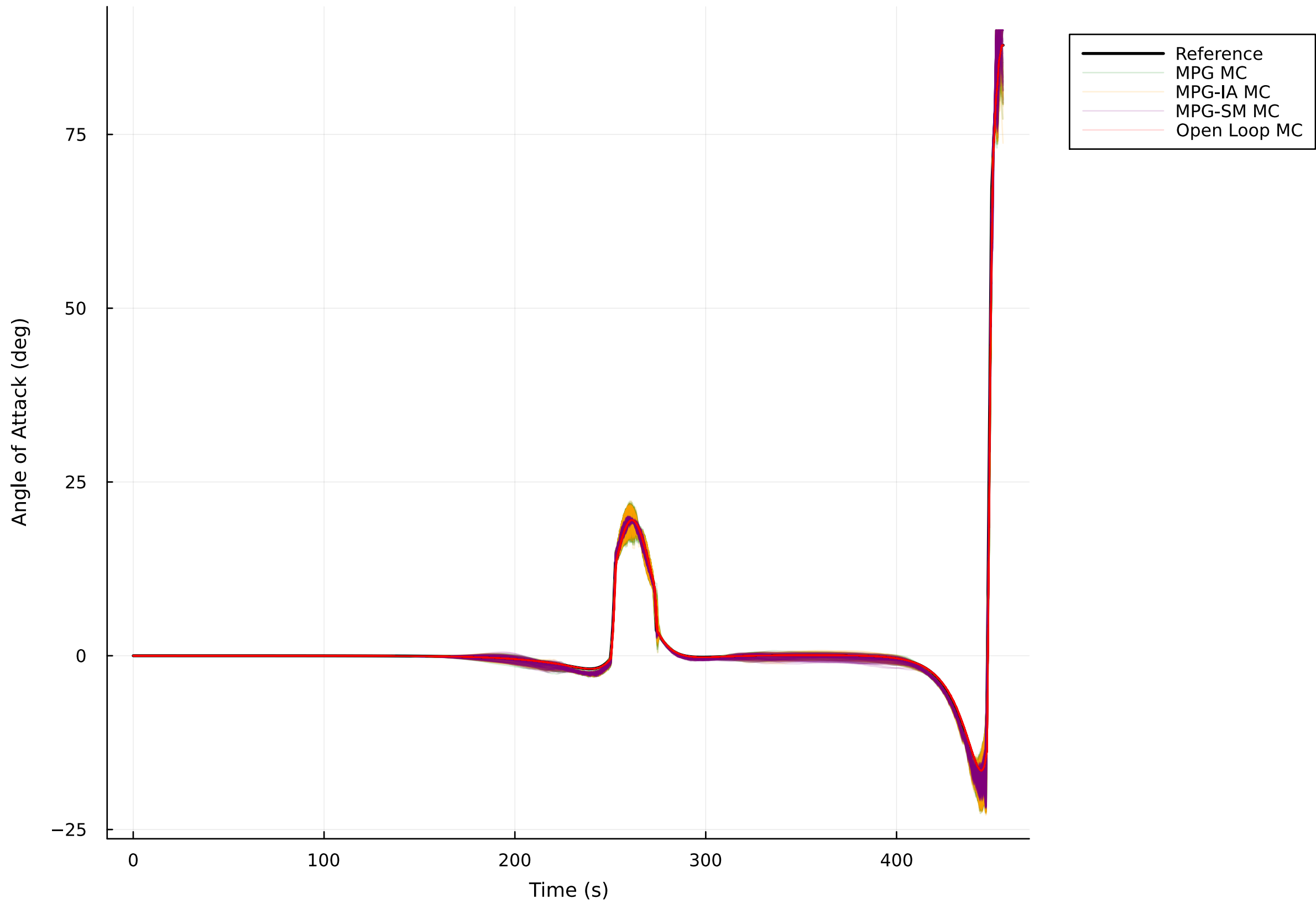
Monte Carlo Simulations: Angle of Attack Profiles
