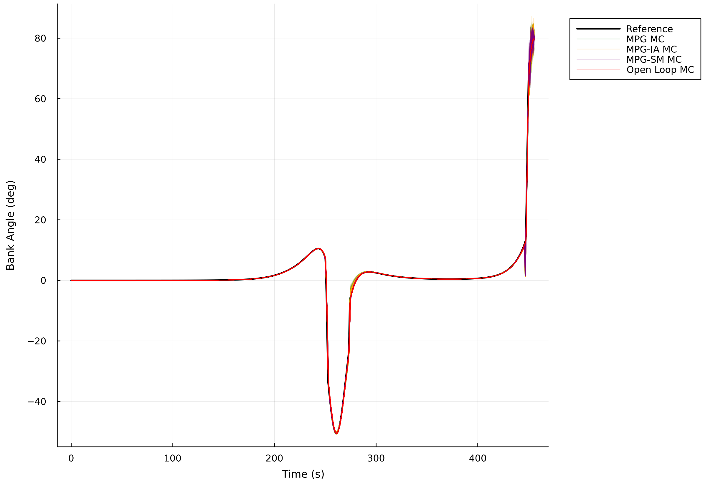
Monte Carlo Simulations: Bank Angle Profiles
