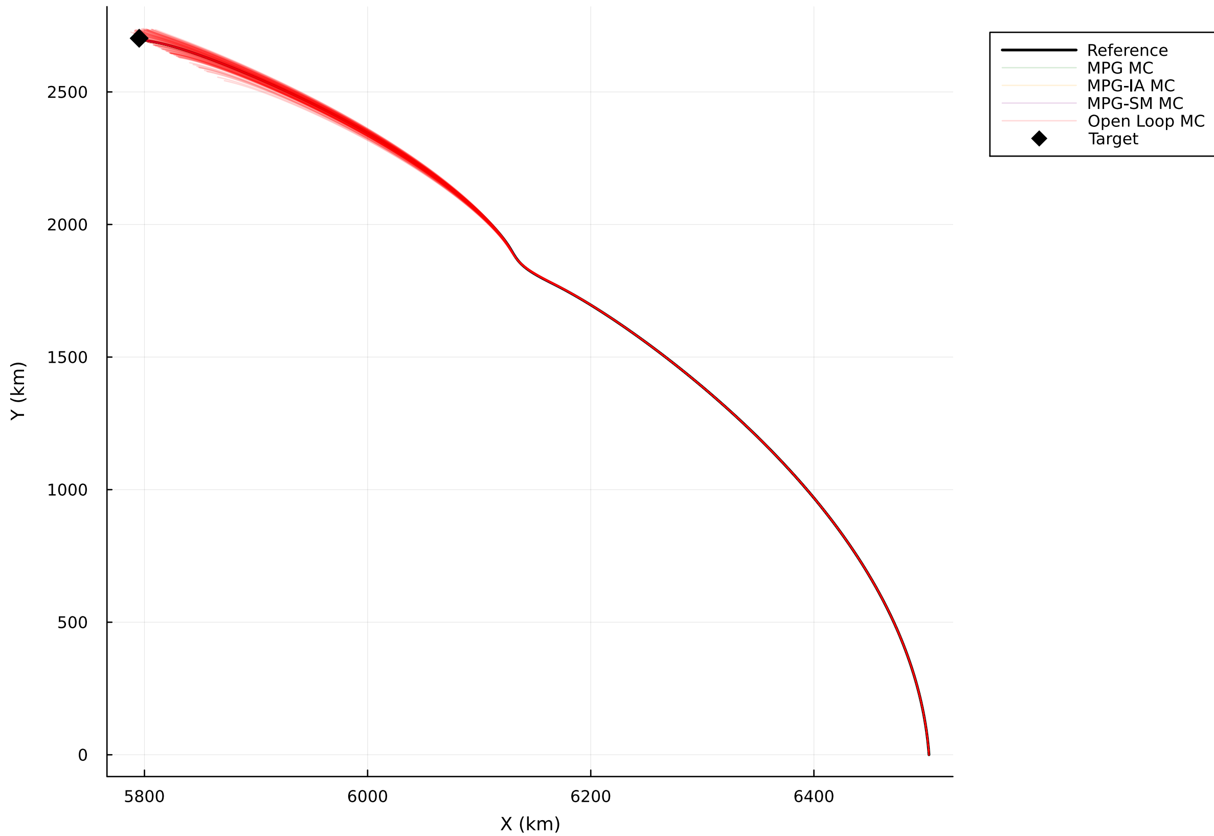
Monte Carlo Simulations: Cartesian Ground Track
