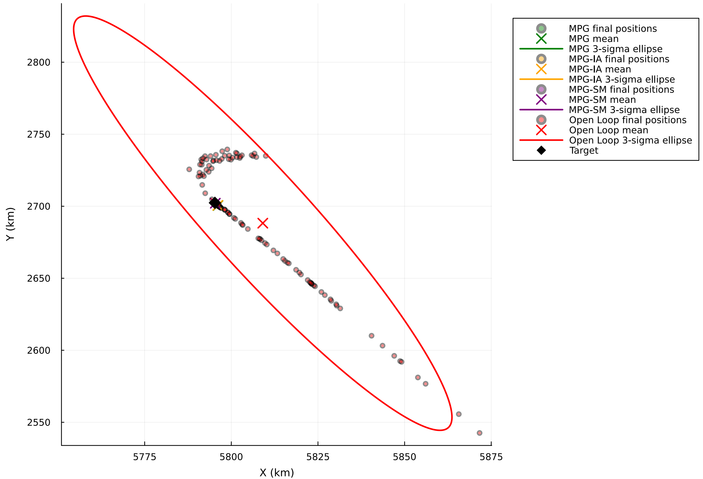
Monte Carlo Simulations: Final Cartesian Locations With 3-Sigma Ellipses
