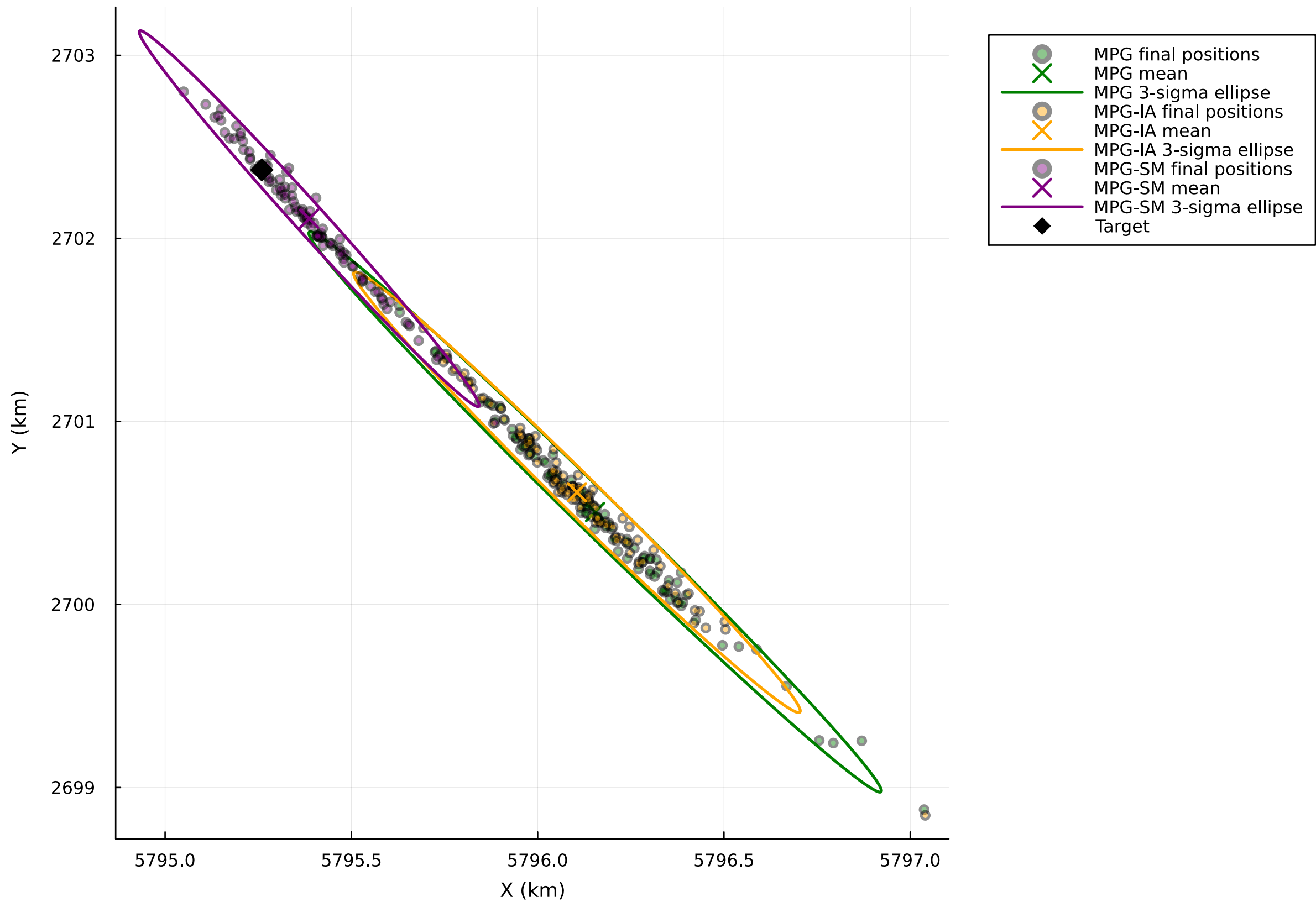
Monte Carlo Simulations: Final Cartesian Locations With 3-Sigma Ellipses (Without Open Loop)
