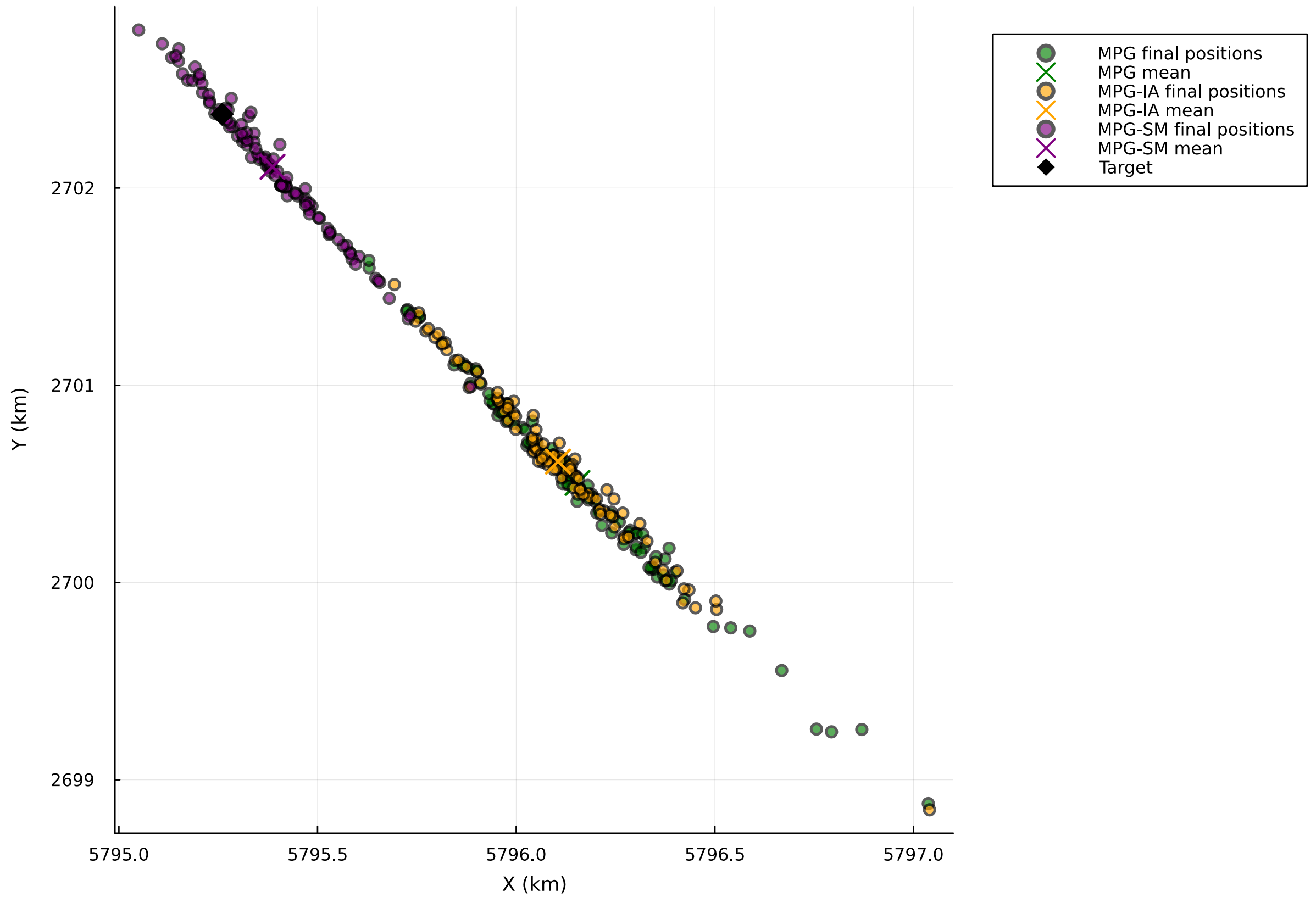
Monte Carlo Simulations: Final Cartesian Locations (Without Open Loop Mean)
