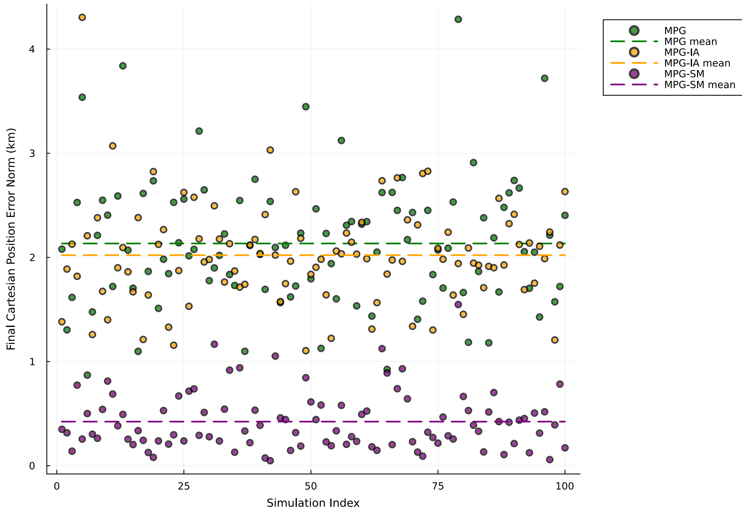
Final Cartesian Position Error Norm (No Open Loop)
