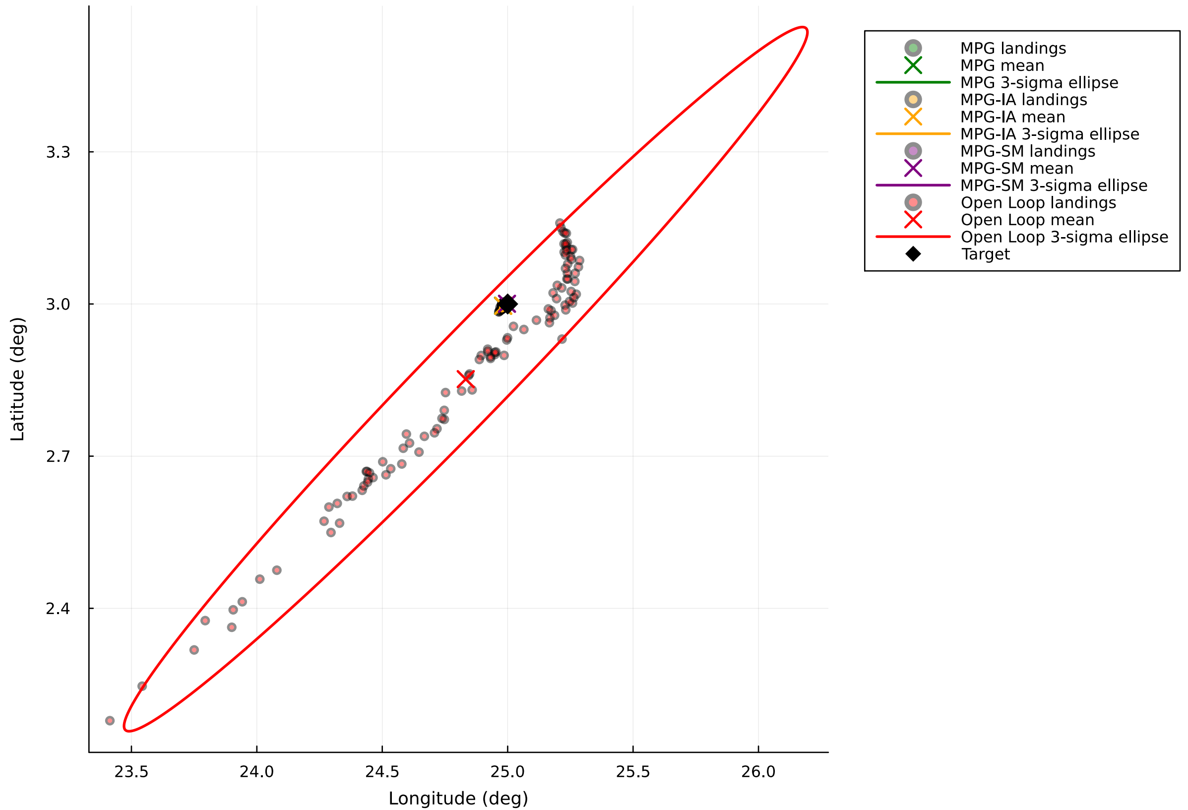
Monte Carlo Simulations: Final Landing Locations With 3-Sigma Ellipses
