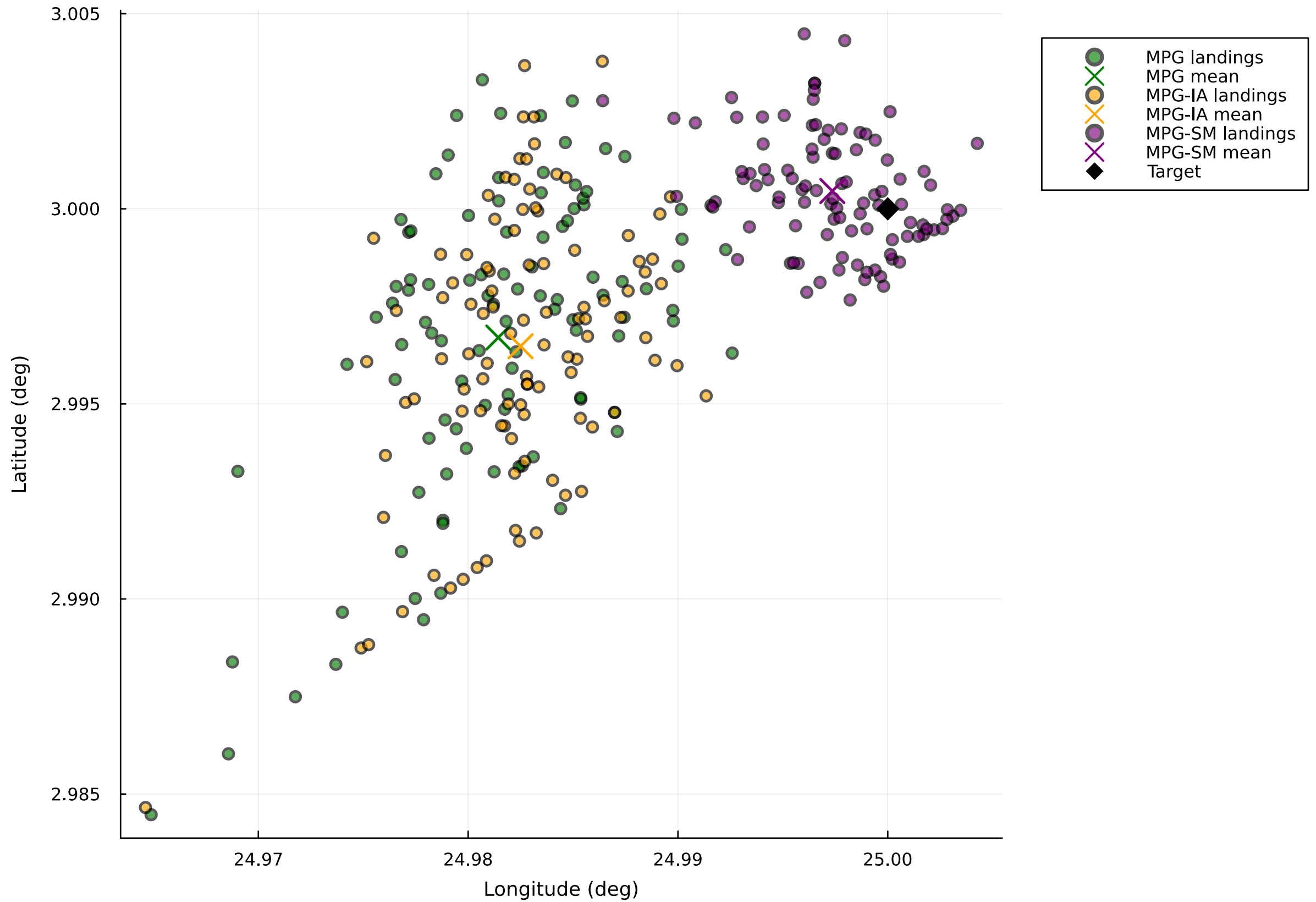
Monte Carlo Simulations: Final Landing Locations (Without Open Loop)
