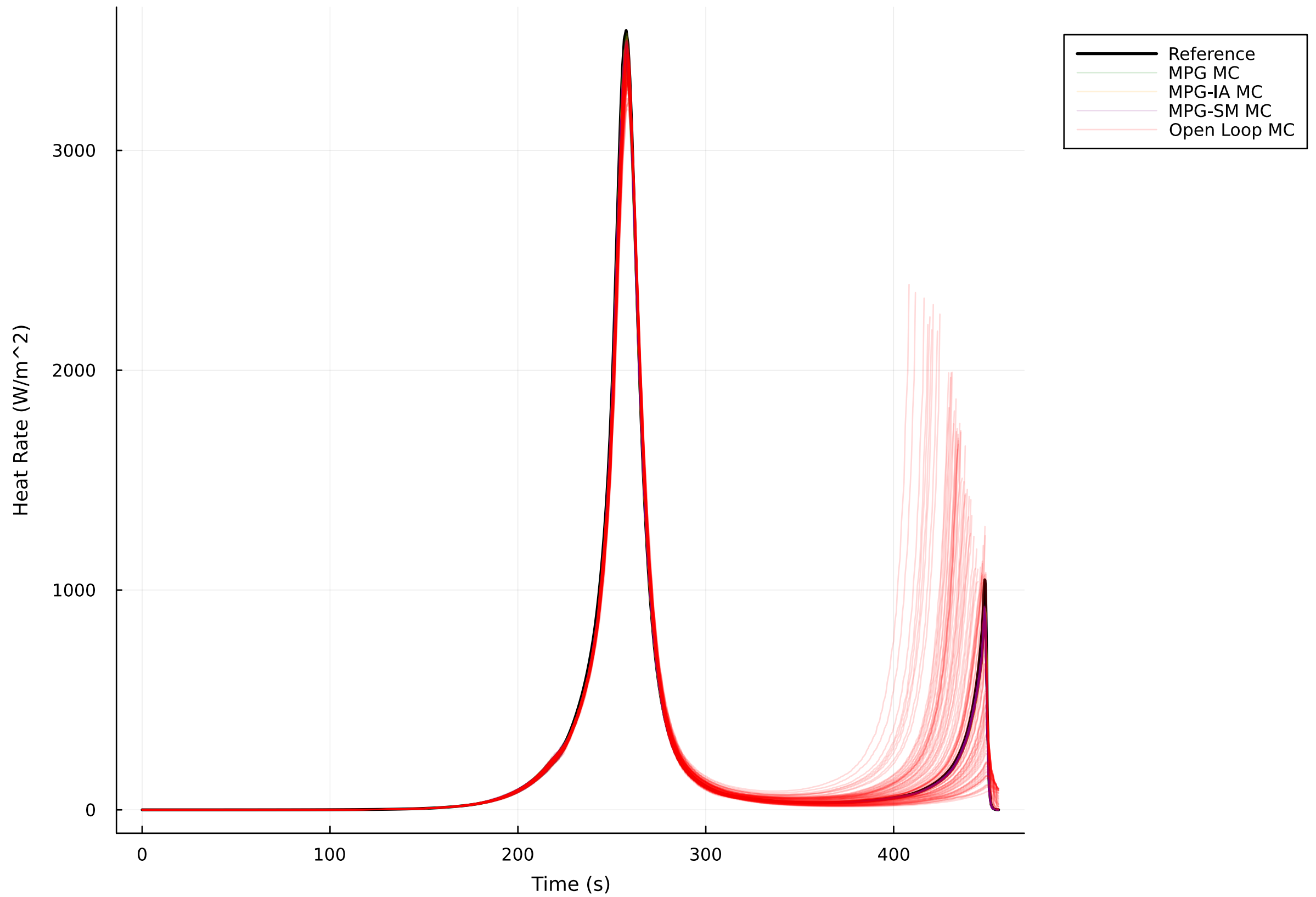
Monte Carlo Simulations: Heat Rate Profiles
