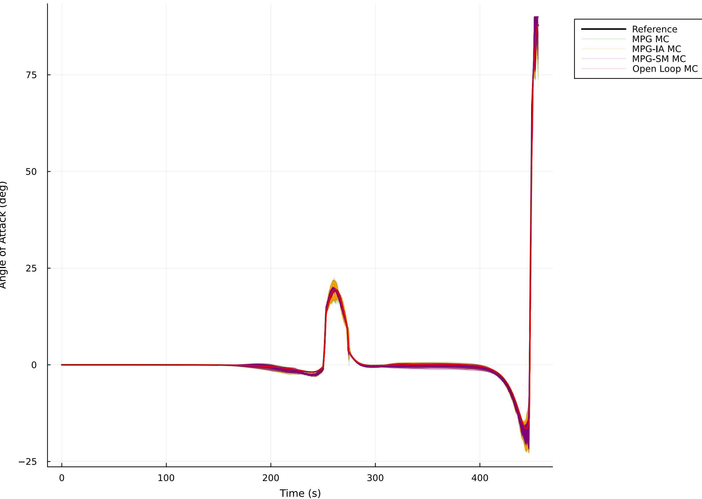
Monte Carlo Simulations: Angle of Attack Profiles
