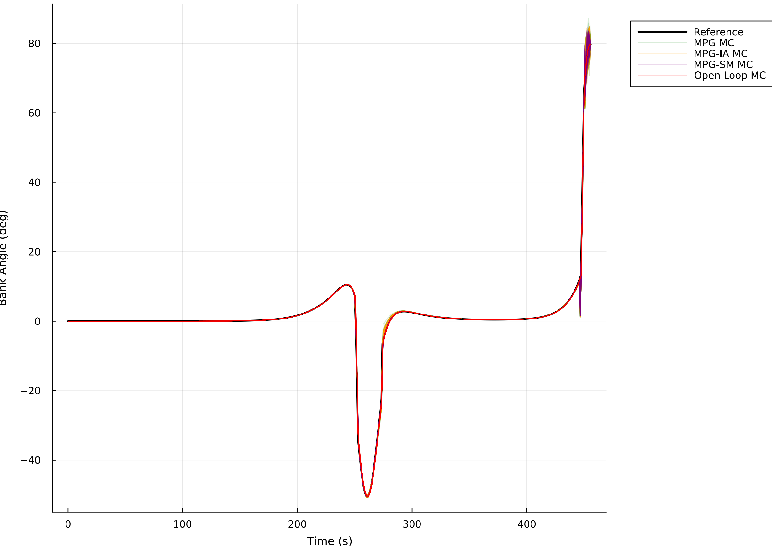
Monte Carlo Simulations: Bank Angle Profiles
