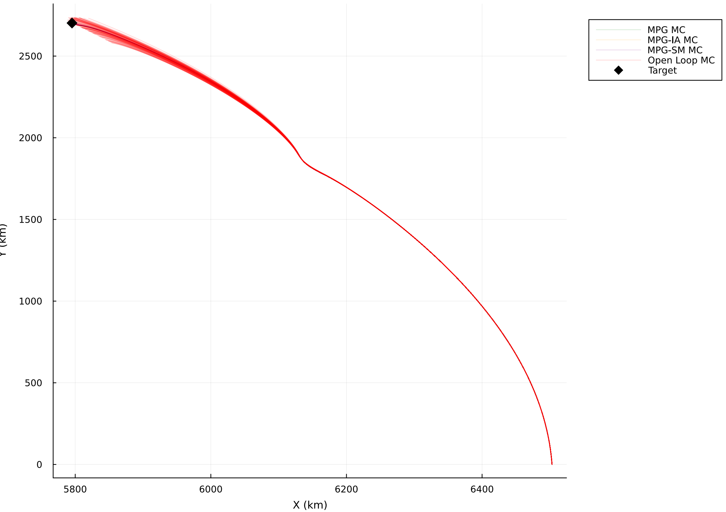
Monte Carlo Simulations: Cartesian Ground Track (No Reference)
