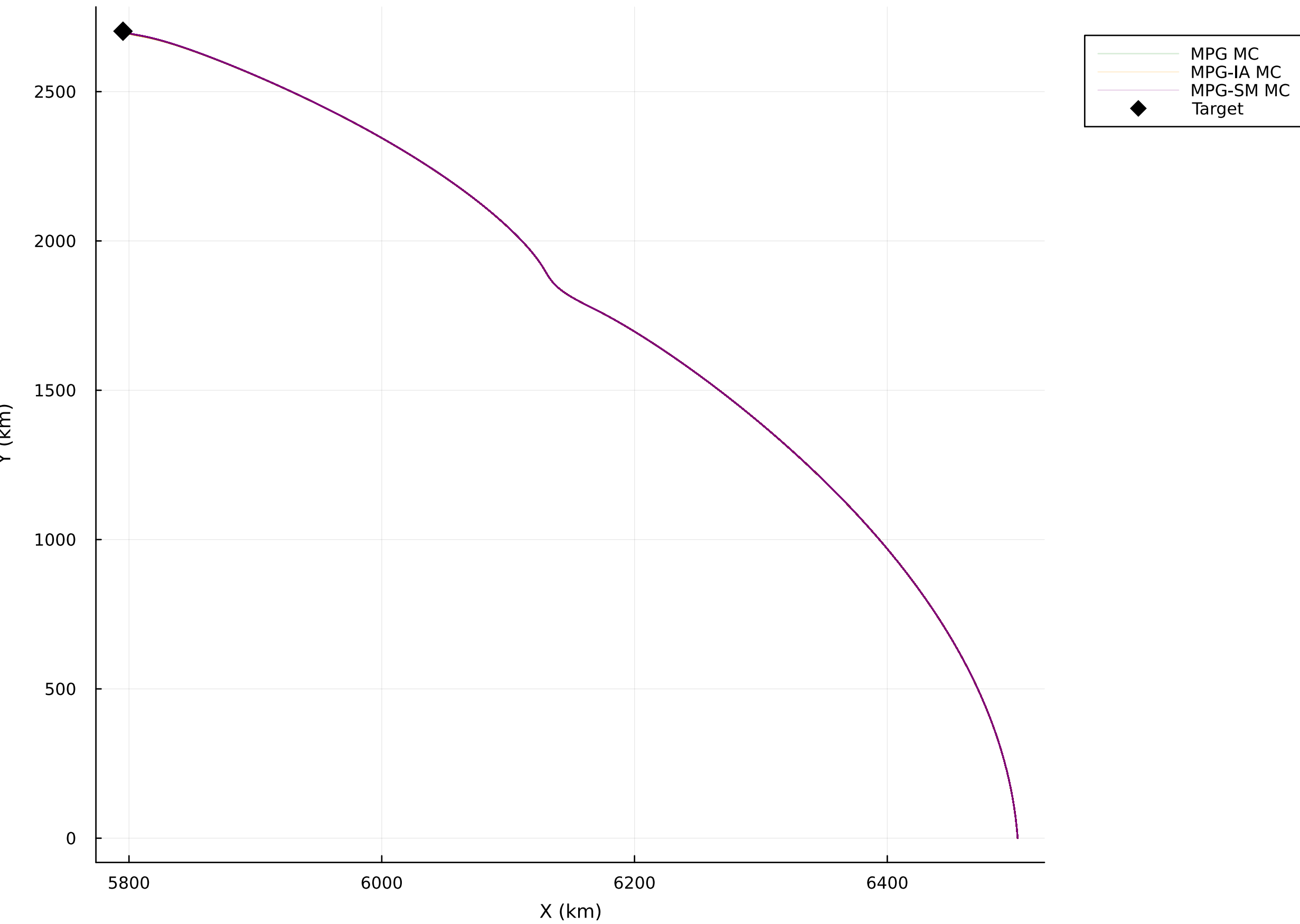
Monte Carlo Simulations: Cartesian Ground Track (NoReference, No Open Loop)
