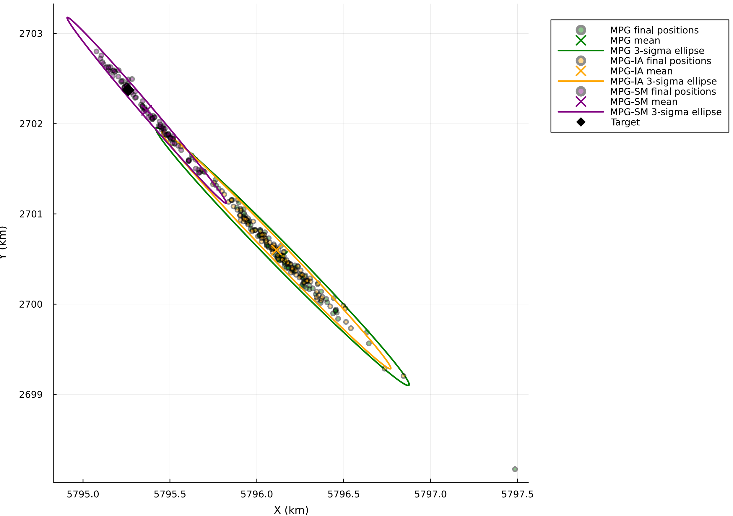
Monte Carlo Simulations: Final Cartesian Locations With 3-Sigma Ellipses (Without Open Loop)
