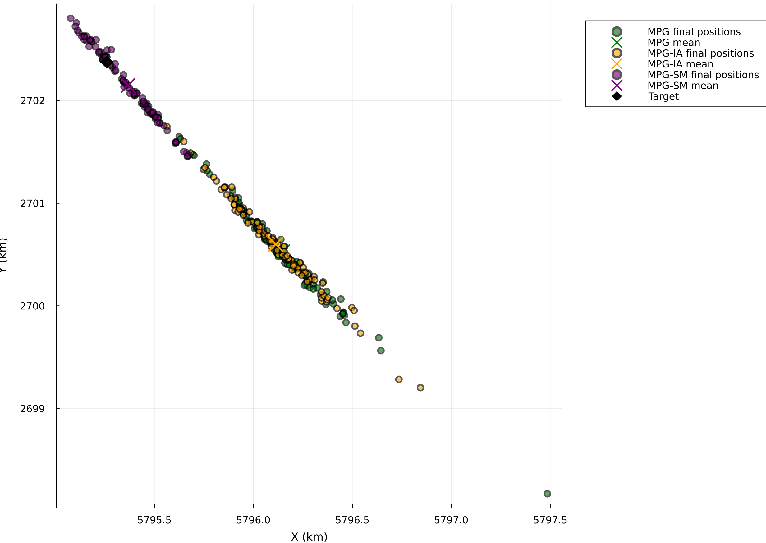
Monte Carlo Simulations: Final Cartesian Locations (Without Open Loop Mean)
